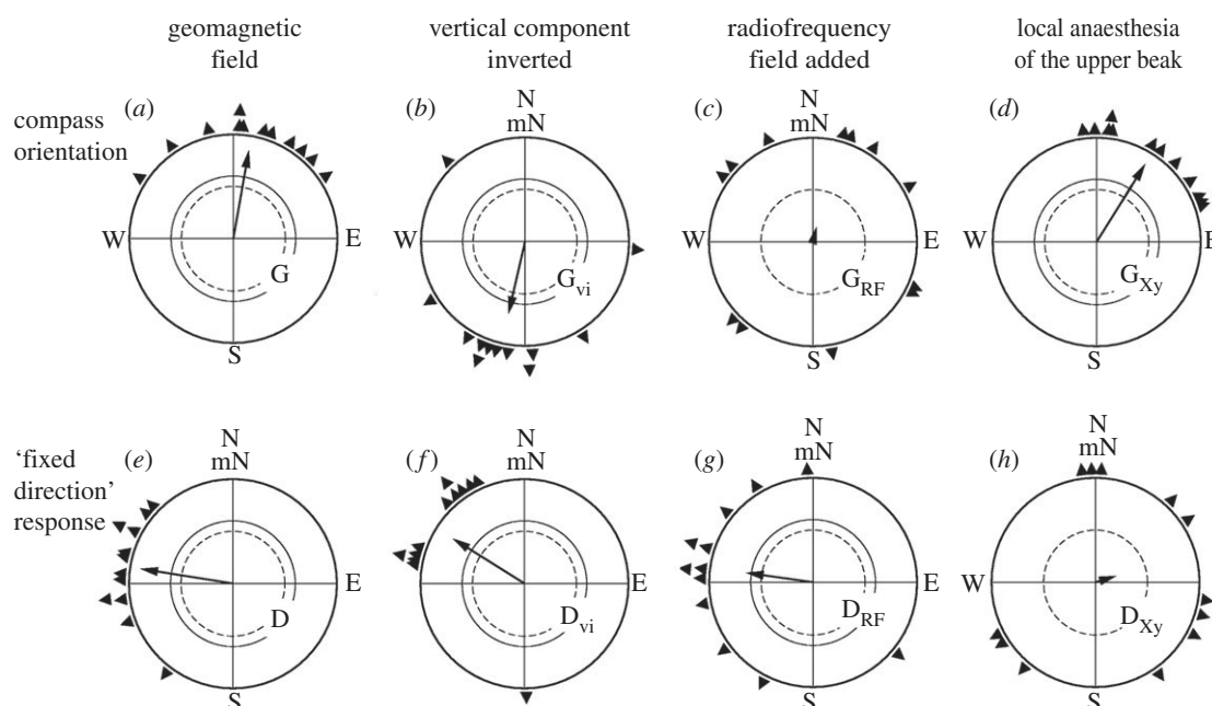
Figure 1. Magnetic compass orientation under green light (G) originating in radical pair processes (a–d), and a ‘fixed direction’ response in total darkness (D), probably originating in magnetite-based receptors in the beak region (e–h). The compass response is not sensitive to the polarity of the magnetic field, but to the axial course of the field lines; it is disrupted by radiofrequency fields, but not affected by anaesthesia up the upper beak. The ‘fixed direction’ response, in contrast, is a polar response; it is not affected by radiofrequency fields, but is disrupted by anaesthesia of the upper beak. The triangles at the periphery of the circle mark the mean directions of individual birds, the arrows indicate the grand mean vector and the inner circles give the 5% (dotted) and the 1% significance border of the Rayleigh test (see [2]).
