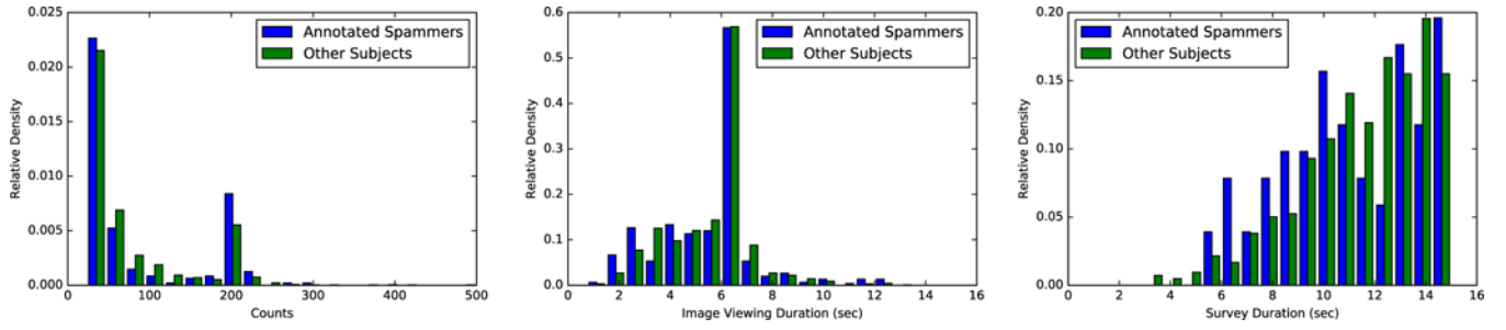
Fig. 6. Normalized histogram of basic statistics including total number of tasks completed and average time duration spent at each of the two stages per task.
