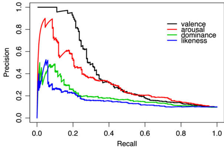
Fig. 8. The agnostic Precision-Recall curve based on manually annotated spammers computed from different affective dimensions: valence, arousal, dominance, and likeness.
