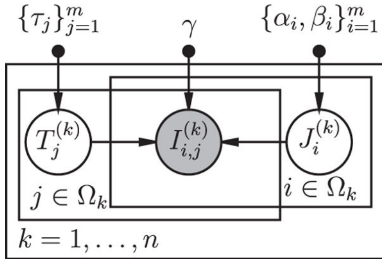
Fig. 4. Probabilistic graphical model of the proposed Gated Latent Beta Allocation.
