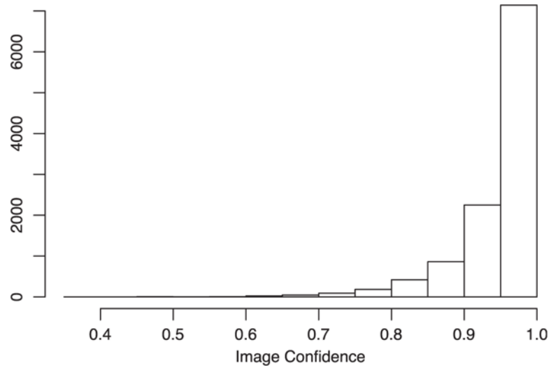
Fig. 10. The histogram of image confidences estimated based on our method. About 85 percent of images have a confidence scores higher than 90 percent.
