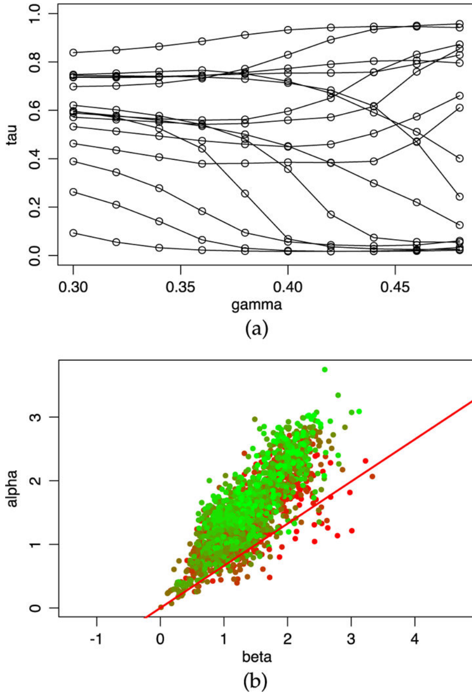
Fig. 5. (a) Reliability scores versus \gamma \in [0.3, 0.48] for the top 15 users who provided the most numbers of ratings. (b) Visualization of the estimated regularity parameters of each worker at a given \gamma . Green dots are for workers with high reliability and red dots for low reliability. The slope of the red line equals \gamma .
