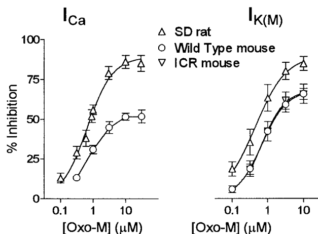
Figure 1. Dose–response curves (mean \pm SEM plus best-fit curve) for Oxo-M inhibition of I_{Ca} and I_{K(M)} in rat and mouse SCG. I_{Ca} , Left , Oxo-M dose–response curves determined after treatment with PTX, thereby isolating the M 1 mAChR-mediated component. n values for each concentration point range from 3 to 7. I_{K(M)} , Right , Oxo-M dose–response curve in wild-type mouse SCG ( n = 9 ) is significantly different from that seen in rat SCG ( n = 4 ; p < 0.001 ). The rat I_{K(M)} dose–response curve data are taken from Haley et al. (1998a), and the rat I_{Ca} dose–response curve data are from Delmas et al. (1998a). Legend applies to both panels. All cells were recorded using the perforated patch method.
