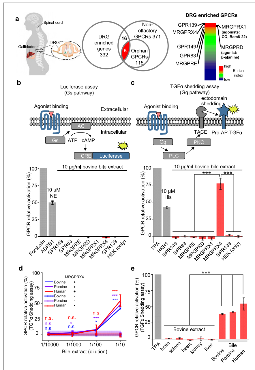
Figure 1. MRGPRX4 is activated by bile extract. (a) Flow chart for the strategy used to identify GPCRs enriched in human DRG. Transcriptome analysis of DRG and other tissues (trigeminal ganglia, brain, colon, liver, lung, skeletal muscle, and testis) revealed 332 transcripts with high expression in the DRG. The top seven GPCRs are listed. See also Supplementary files 1 and 2 . Gene expression data were obtained from Flegel et al. (2013) . (b and c) Activation of MRGPRX4 by bovine bile extract. The diagrams at the top depict the reporter gene assays used to measure GPCR activation via Gs-dependent (b) and Gq-dependent (c) pathways. The seven GPCRs identified in (a) were tested, revealing that MRGPRX4-expressing HEK293T cells are activated by bile extract via the Gq-dependent pathway. Forskolin and TPA were used as positive controls for activating Gs- and Gq-dependent signaling, respectively. The responses obtained from the tested GPCRs were normalized to the responses induced by respective positive controls. As positive controls for detecting GPCR activation, separate cells were transfected with ADRB1 and stimulated with 10 µM norepinephrine (NE) (b) or transfected with HRH1 and stimulated with 10 µM histamine (His) (c). ‘HEK (only)’ refers to non-transfected cells. n = 3 experiments performed in triplicate. (d) Concentration-response curve for the activation of MRGPRX4 by bovine bile extract, porcine bile extract, and human bile measured using the TGFα shedding assay. The bovine and porcine bile extract solutions were diluted 1 :10 from a 100 µg/ml stock solution, and the human bile solution was diluted 1:10 from crude human bile. n = 2 Figure 1 continued on next page
