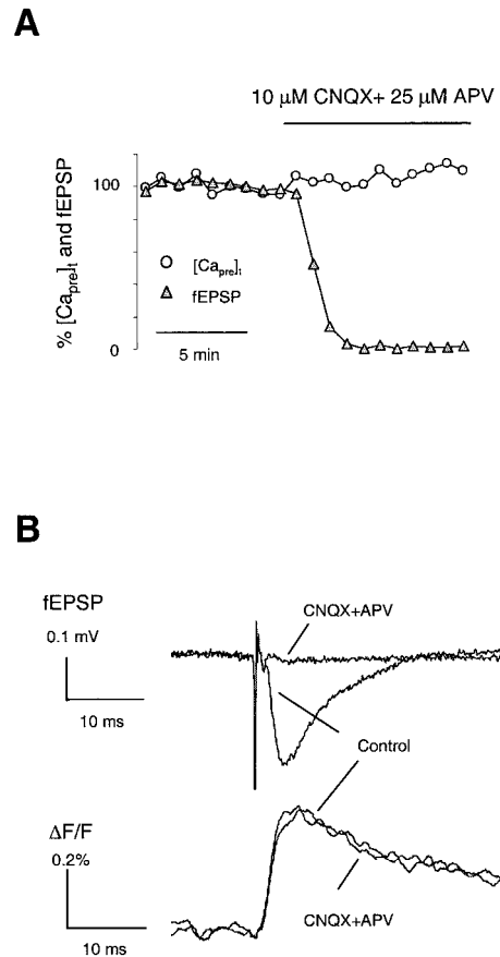
Figure 1. Selective loading of presynaptic terminals with the Ca 2+ indicator Magnesium Green AM at the mouse hippocampal synapse. A , Time courses of mean amplitudes of presynaptic Ca 2+ transient ( [Ca_{pre}]_t ) and fEPSPs under control saline conditions and during application of glutamate receptor antagonists CNQX and D-APV in a typical experiment. Blockade of the fEPSP did not alter the evoked fluorescence signal, indicating a presynaptic origin. B , Superimposed sample traces of the optical Ca 2+ \Delta F/F signal and the fEPSP taken during the steady-state response period in control saline and after application of the glutamate receptor antagonists. The Ca 2+ \Delta F/F trace is an average of three consecutive samples. CNQX and D-APV abolished the fEPSP but did not change the \Delta F/F , indicating that the measured Ca 2+ signal was purely presynaptic.
