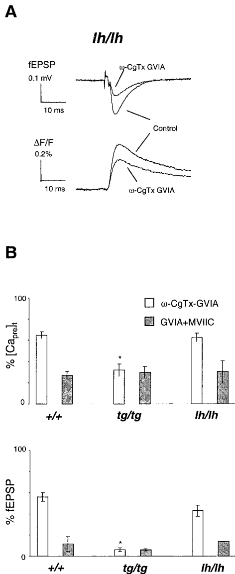
Figure 3. Presynaptic effects of \text{Ca}^{2+} channel toxins on [\text{Ca}^{2+}]_{\text{pre,t}} and fEPSP are similar in lh/lh and +/+ mice. A , Sample traces of [\text{Ca}^{2+}]_{\text{pre,t}} and fEPSP in response to \omega -CgTx GVIA in a typical experiment from a lh/lh mouse. \omega -CgTx GVIA ( 1 \mu\text{M} ) decreased the [\text{Ca}^{2+}]_{\text{pre,t}} to the level similar to that in +/+ slices, and fEPSP was partially reduced. B , Summary data for the effects of \text{Ca}^{2+} channel toxins on [\text{Ca}^{2+}]_{\text{pre,t}} and fEPSP from +/+ , tg/tg , and lh/lh mice. There was a significant difference in the presynaptic \text{Ca}^{2+} influx profile between +/+ and tg/tg mice (for both N- [\text{Ca}^{2+}]_{\text{pre,t}} and P/Q- [\text{Ca}^{2+}]_{\text{pre,t}} ; paired two-tailed t test; p < 0.005 ) but not between +/+ and lh/lh mice.
