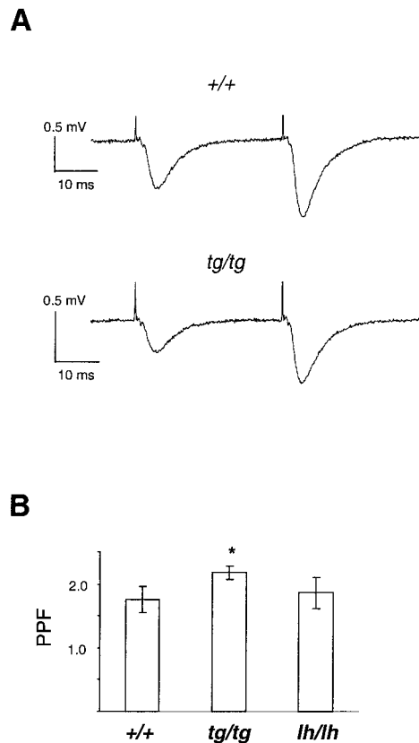
Figure 5. Increased paired-pulse facilitation in tg/tg mouse. A , Representative sample traces of the fEPSP in response to paired-pulse stimulation in +/+ and tg/tg mice. B , Summary PPF data from +/+ , tg/tg , and lh/lh mouse slices. PPF was similar in lh/lh and +/+ mice. PPF in tg/tg mice was significantly larger than in +/+ mice, suggesting a reduced level of neurotransmitter release at tg/tg synapses.
