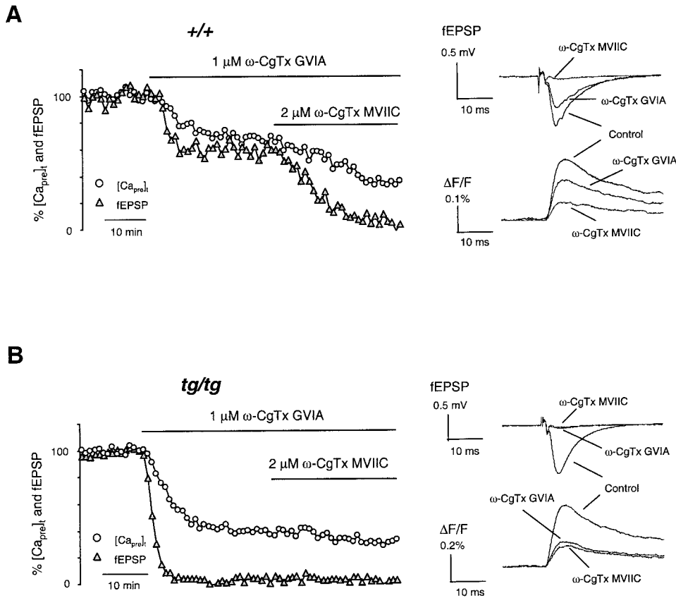
Figure 2. Differential effects of Ca 2+ channel toxins on [\text{Ca}_{\text{pre}}]_t and fEPSP in +/+ and tg/tg mice. A , Time courses of [\text{Ca}_{\text{pre}}]_t and fEPSP in response to \omega\text{-CgTx GVIA} and \omega\text{-CgTx MVIIC} in a representative experiment from +/+ mouse. Blockade of N-type Ca 2+ currents with 1 \mu\text{M} \omega\text{-CgTx GVIA} partially blocked synaptic transmission (~35% of the total Ca 2+ influx). In the presence of \omega\text{-CgTx GVIA} , 2 \mu\text{M} \omega\text{-CgTx MVIIC} further reduced [\text{Ca}_{\text{pre}}]_t by ~40% and completely abolished fEPSP, indicating the involvement of P/Q-type channels in neurotransmitter release as well. Inset shows sample traces taken during steady-state periods in the control solution and after application of \omega\text{-CgTx GVIA} and \omega\text{-CgTx MVIIC} . B , Time courses of [\text{Ca}_{\text{pre}}]_t and fEPSP in response to \omega\text{-CgTx GVIA} and \omega\text{-CgTx MVIIC} in a typical experiment from tg/tg mouse. In contrast to +/+ slices, \omega\text{-CgTx GVIA} primarily reduced [\text{Ca}_{\text{pre}}]_t (by ~70%) and completely eliminated synaptic transmission. Further application of \omega\text{-CgTx MVIIC} revealed a small amount of P/Q-type current (~6%). This indicates that mutation of the \alpha_{1A} subunit in tg/tg mice severely compromises the function of P/Q-type Ca 2+ channels, resulting in a heavy reliance of neurotransmitter release on N-type Ca 2+ channels. Inset shows sample traces taken in the steady state of control solutions and after application of \omega\text{-CgTx GVIA} and \omega\text{-CgTx MVIIC} .
