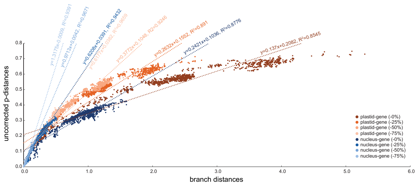
Fig. 6. —Saturation plot that shows the relationship between taxon–taxon uncorrected p -distances and (corrected) branch distances for both plastid-gene and nucleus-gene data sets after 0%, 25%, 50%, and 75% of the fastest-evolving sites have been removed.
