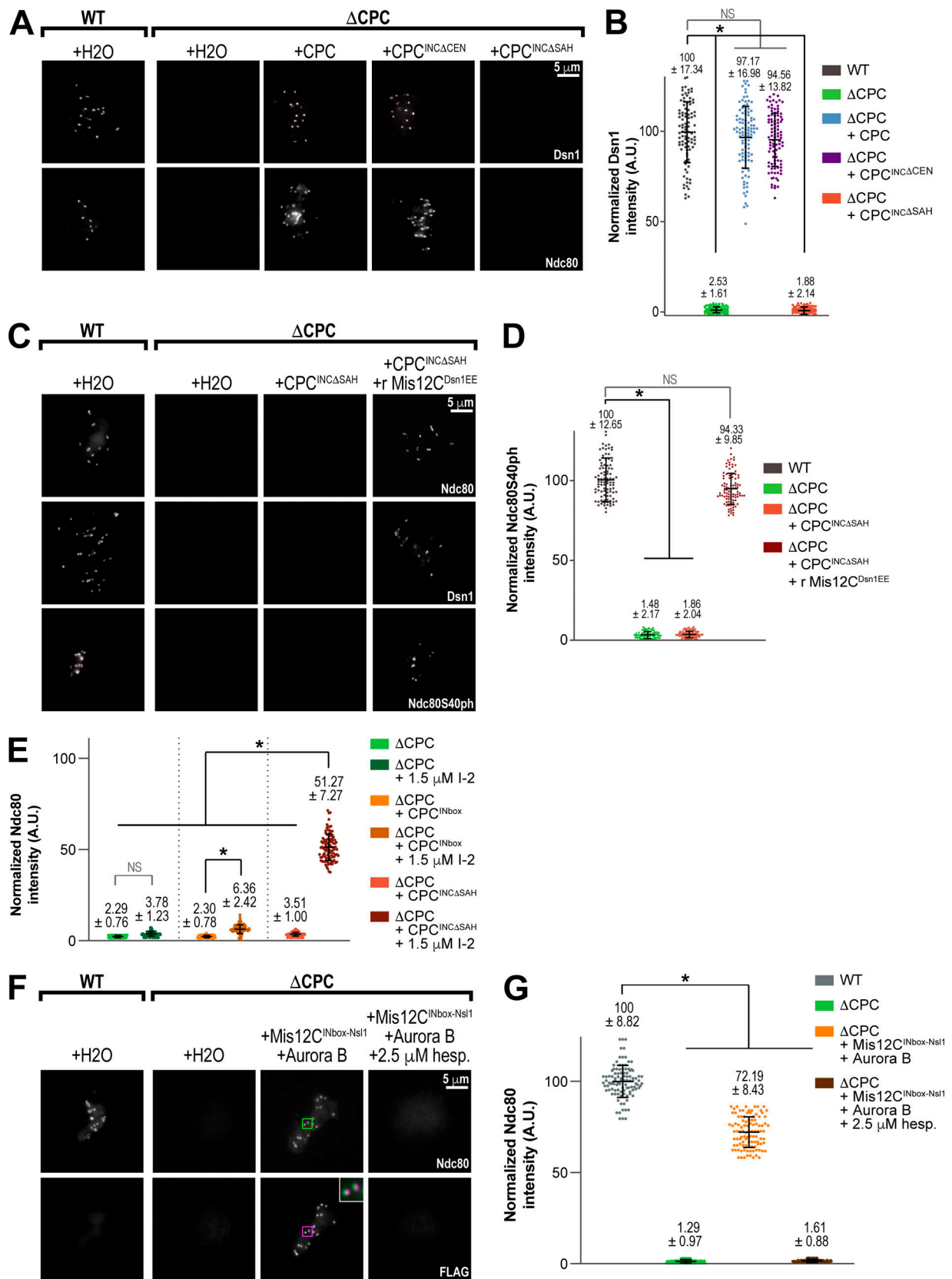
Figure 3. The SAH domain of INCENP is critical for kinetochore assembly. (A) Representative immunofluorescence images of replicated chromosomes in WT and ΔCPC metaphase extracts reconstituted with CPC containing the indicated INCENP construct with anti-INCENP antibody added for the INC ΔCEN sample to ensure kinase activation. Samples contained 33 μM nocodazole. Chromosomes were stained for Dsn1 and Ndc80. (B) Quantification of fluorescence intensity of Dsn1 on replicated chromosomes in WT or ΔCPC metaphase extracts reconstituted with indicated CPC conditions
