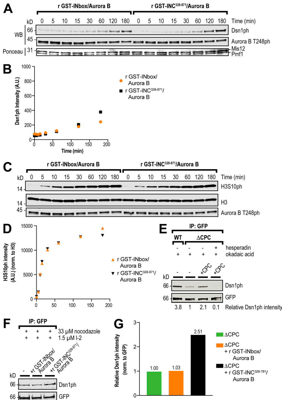
Figure 4. The central region promotes Dsn1 phosphorylation by Aurora B. (A) In vitro kinase assay for Dsn1 phosphorylation. Purified Xenopus recombinant (r) Mis12C was incubated with pre-activated recombinant GST-INbox-His 6 -Aurora B kinase or recombinant GST-INC 328-871 -His 6 -Aurora B for the indicated times, and phosphorylation was assessed by Western blot (WB) using a phospho-specific antibody to Ser77 of Dsn1. (B) Quantification of kinase assay for Dsn1 phosphorylation shown in A. A.U., arbitrary units. (C) In vitro kinase assay for histone H3 phosphorylation (H3S10ph). Purified Xenopus recombinant H3-H4 was incubated with preactivated recombinant GST-INbox-His 6 -Aurora B kinase or recombinant GST-INC 328-871 -His 6 -Aurora B for the indicated times, and phosphorylation was assessed by Western blot using a phospho-specific antibody for H3S10ph. (D) Quantification of kinase assay for H3S10 phosphorylation shown in C. (E) Western blot for phosphorylation of Dsn1 in samples of immunoprecipitated (IP) recombinant Mis12 Dsn1-LAP complex from WT and ΔCPC metaphase extracts, in indicated CPC conditions, in the presence of nocodazole, okadaic acid, and hesperadin as specified. Normalized phosphorylation levels are indicated below. (F) Western blot for phosphorylation of Dsn1 in samples of immunoprecipitated Mis12 Dsn1-LAP complex expressed from mRNAs in ΔCPC metaphase extracts, in indicated CPC conditions. Recombinant GST-INbox-His 6 -Aurora B or recombinant GST-INC 328-871 -His 6 -Aurora B were activated with anti-INCENP beads in the presence of nocodazole and I-2. (G) Quantification of phosphorylation of Dsn1 from samples shown in C, normalized to GFP.
