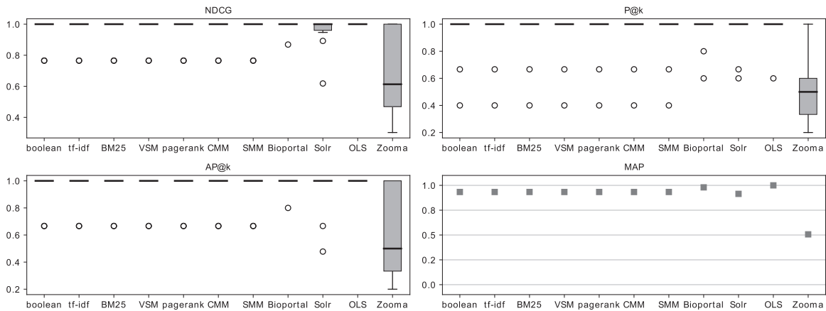
Figure 7. NDCG, P@k, AP@k and MAP results for the 10 query collection, considering exact matches only, against the PGT.
