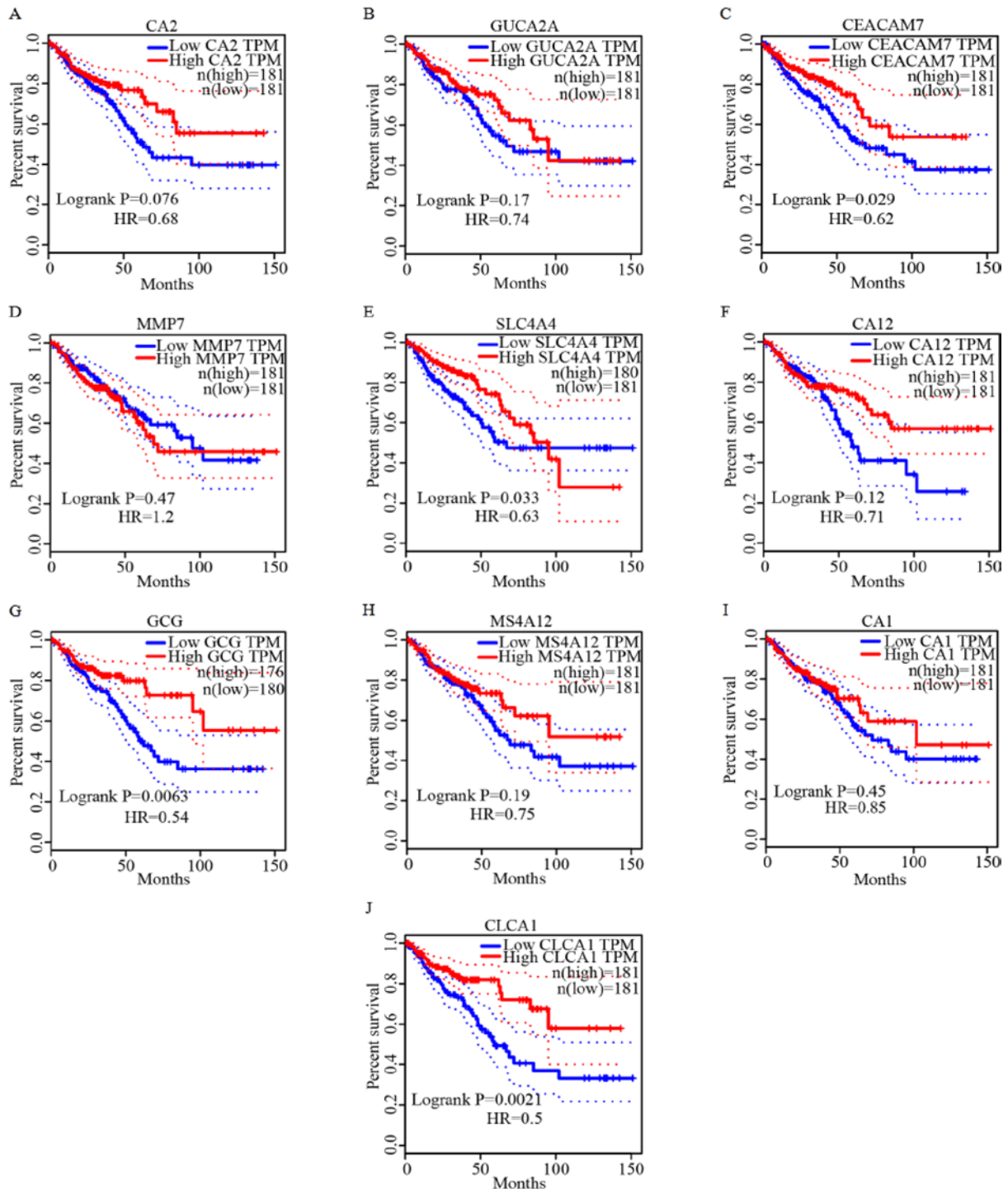
Figure 6. Survival curves of overall survival analysis of ten key genes. Survival curves of overall survival time of (A) CA2, (B) GUCA2A, (C) CEACAM7, (D) MMP7, (E) SLC4A4, (F) CA12, (G) GCG, (H) MS4A12, (I) CA1 and (J) CLCA1. CA2, carbonic anhydrase 2; GUCA2A, guanylate cyclase activator 2A; CEACAM7, carcinoembryonic antigen-related cell adhesion molecule 7; MMP7, matrix metalloproteinase-7; SLC4A4, solute carrier family 4 member 4; GCG, glucagon; MS4A12, membrane-spanning 4-domains subfamily A member 12; CA2, carbonic anhydrase 2; CLCA1, calcium-activated chloride channel regulator 1; TPM, transcripts per million.
