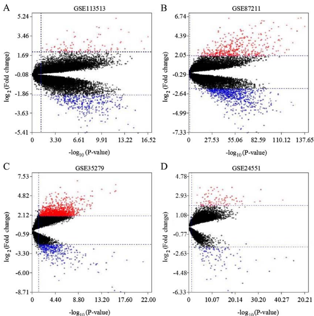
Figure 3. Volcano plot of DEGs in datasets GSE113513, GSE87211, GSE35279 and GSE24551. Red dots represent upregulated DEGs and blue dots represent downregulated DEGs with a threshold of \log_2\text{FC} \geq 2.0 and adjusted P < 0.05 in datasets (A) GSE113513, (B) GSE87211, (C) GSE35279 and (D) GSE24551. DEGs, differentially expressed genes; FC, fold change.
