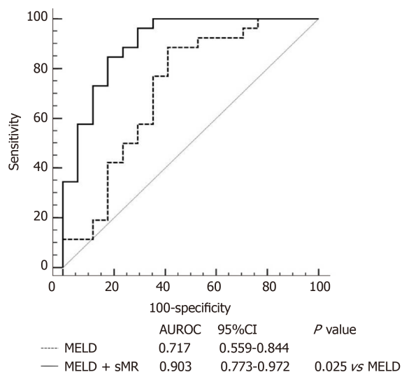
Figure 5 Areas under the receiver operating characteristics curves of model for end-stage liver disease score alone and model for end-stage liver disease score plus serum soluble mannose receptor. AUROC: Area under the receiver operating characteristics curve; CI: Confidence interval; MELD: Model for end-stage liver disease; sMR: Soluble mannose receptor.
