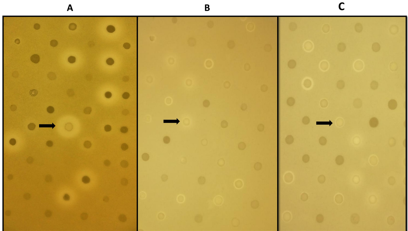
Fig 1. Representative images of the results obtained during the screen of 100 CoNS strains for antimicrobial activity. CoNS were replicated from master stock 96 well plates onto BHI agar using a 96-pin replicator. Plates were incubated at 37°C overnight after which they were overlaid with sloppy agar containing relevant indicator bacteria. For the plates shown the indicators used were (A) M. luteus DSM1790, (B) S. aureus NCDO1499 and (C) S. pseudintermedius DSM21284. The arrows indicate the position of S. capitis CIT060 on the plates.
