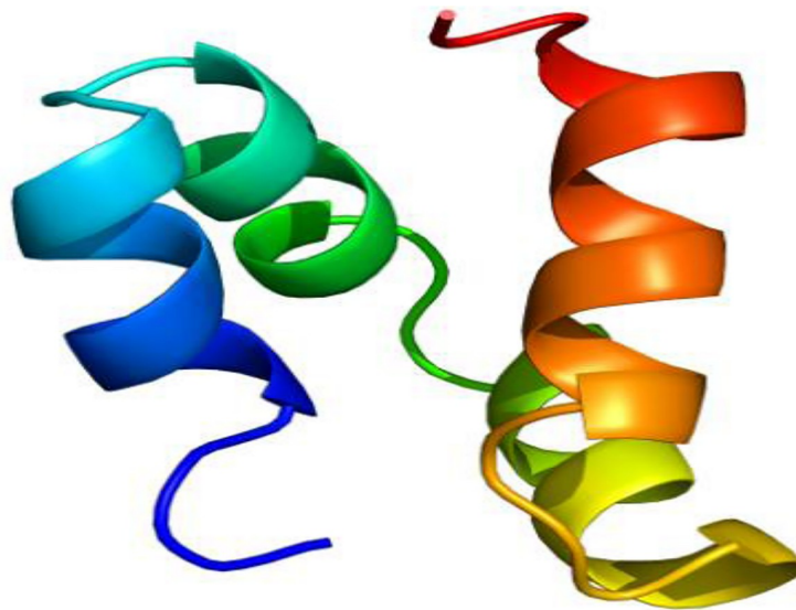
Fig 5. Putative three-dimensional structure of capidermicin. A rainbow colour scheme is used to indicate the N-terminus in blue, and the C-terminus in red. The structure was generated using Phyre2.
