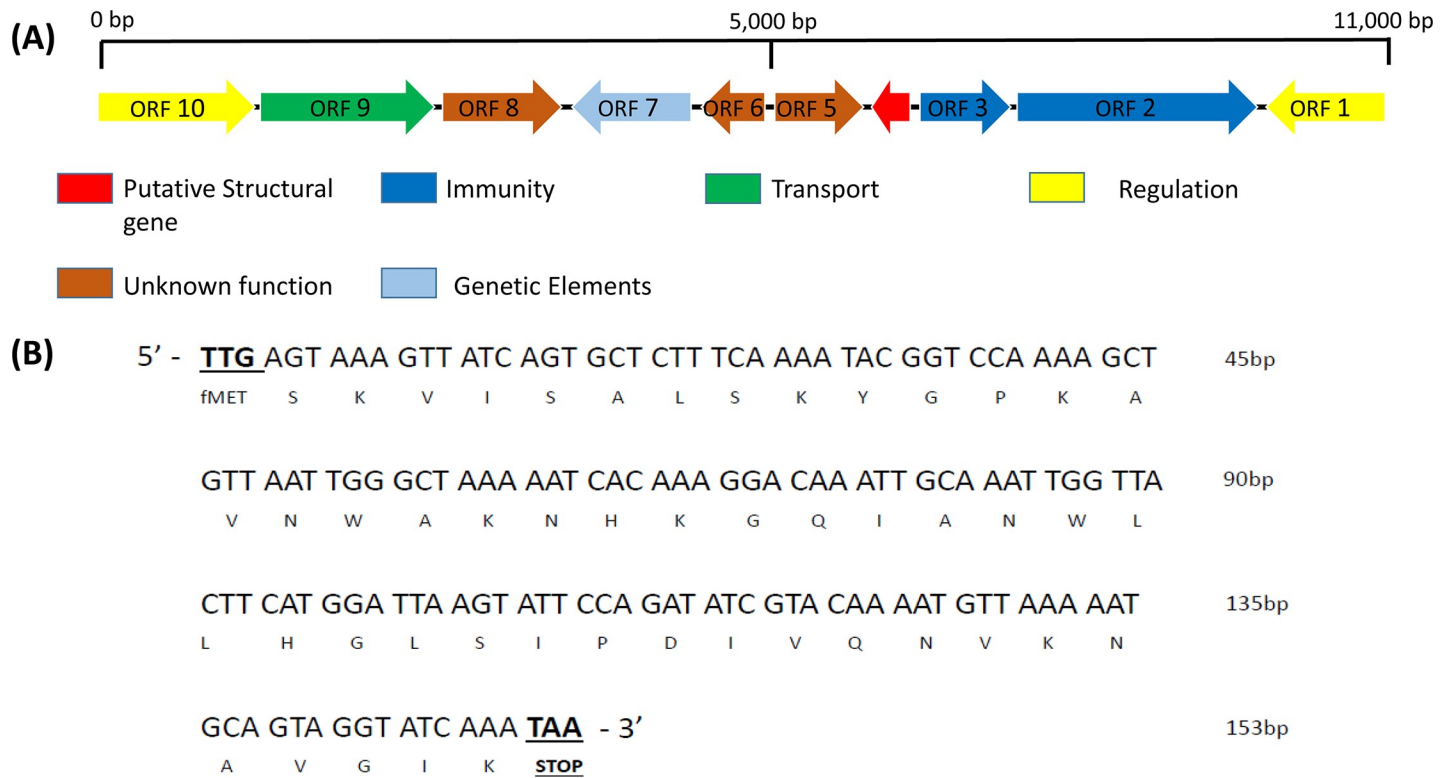
Fig 3. (A) Organisation of the genomic region that is predicted to encode capidermicin. Open reading frames (ORFs)/genes are coloured according to the predicted function. (B) The nucleotide sequence of the 153 bp ORF4 that is predicted to encode capidermicin. The deduced amino acid sequence is shown under the DNA sequence. The start and stop codon, TTG and TAA, respectively, are shown in bold and underlined.
