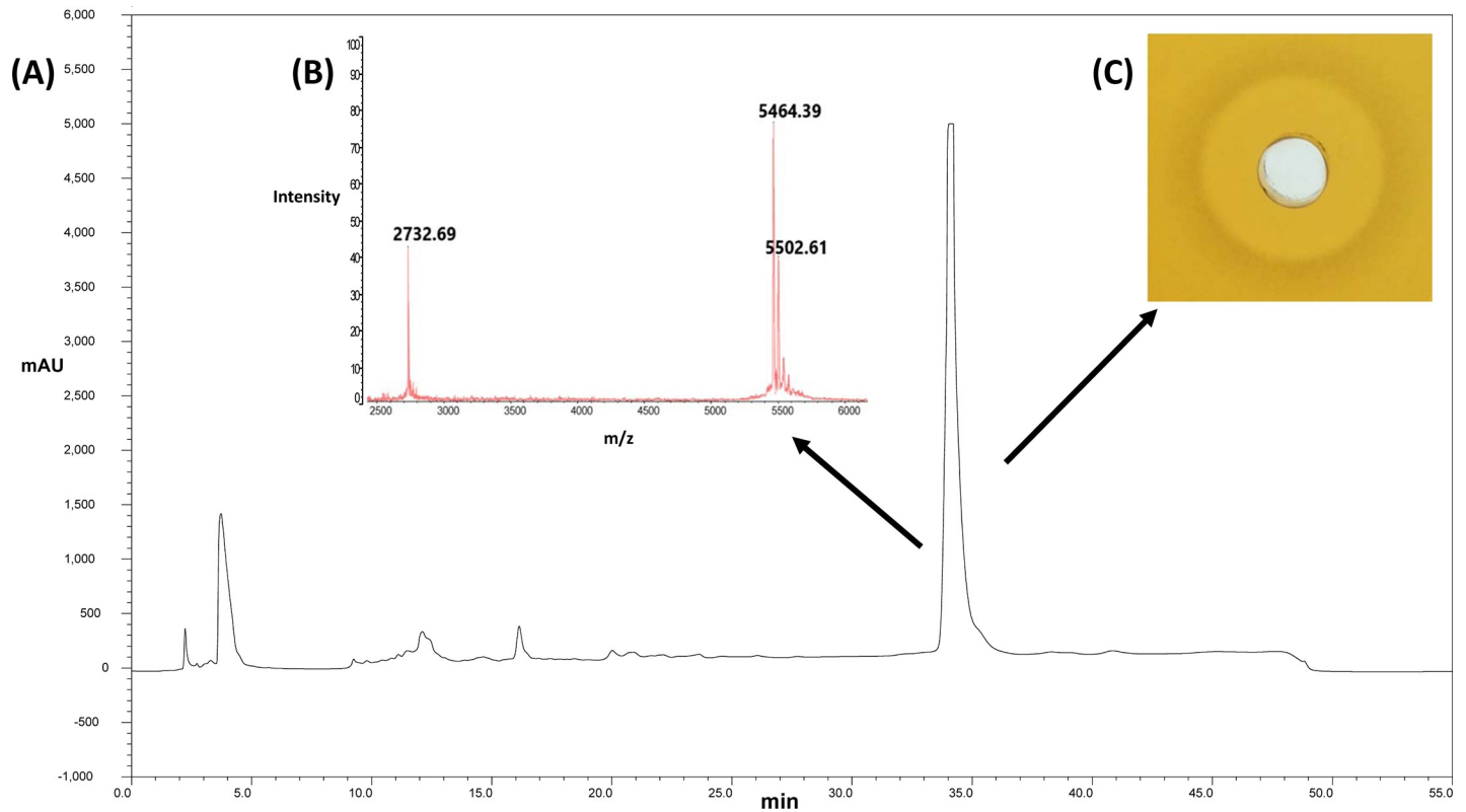
Fig 2. (A) Reversed-phase high performance liquid chromatography (RP-HPLC) profile for the purification of capidermicin using a Phenomenex C12 reverse-phase column, at a flow rate of 2ml/min. (B) MALDI-TOF Mass Spectrometry of lyophilized capidermicin revealed a mass of 5,464 Da. MALDI TOF MS chromatogram above indicates the presence of capidermicin (5464.39) and the K + adduct ion (5502.61) and the doubly charged ion (2732.69) (2732 x 2 = 5464). (C) Antimicrobial activity of HPLC bioactive fractions was determined using well diffusion assay using L. lactis HP as the indicator strain. GM17 agar was seeded with L. lactis HP, wells were bored, 50µL of the HPLC fraction was added to the well, and plates were incubated at 30°C for 16 hours.
