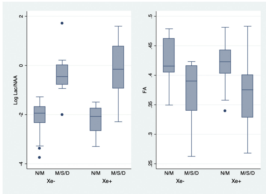
Fig. 3. Plot of log Lac/NAA (N = 69) and FA (N = 66) values and outcome at 2–3 years of age by treatment group. Two group t -test of means of Lac/NAA on the log scale, in normal outcome/mild disability and moderate/severe disability/deaths groups in Xe + group, P < .001 and Xe- groups, P < .001; Two group t -test of means of FA, in normal outcome/mild disability and moderate/severe disability/deaths groups in Xe+, P < .001 and Xe- groups, P < 0.001.
