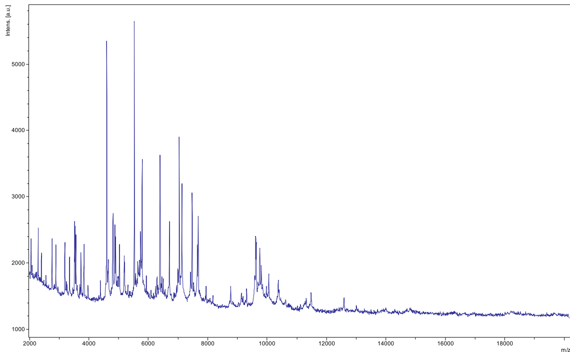
FIG. 1. MALDI-TOF MS reference mass spectrum of Parabacteroides massiliensis sp. nov. Spectra from 12 individual colonies were compared and a reference spectrum was generated.
