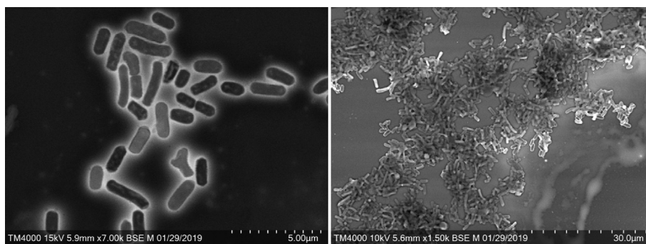
FIG. 3. Scanning electron micrograph of Parabacteroides massiliensis strain Marseille-P2231 T using TM4000 microscope from HITACHI. Scale bar and acquisition settings are shown on the original micrograph.
