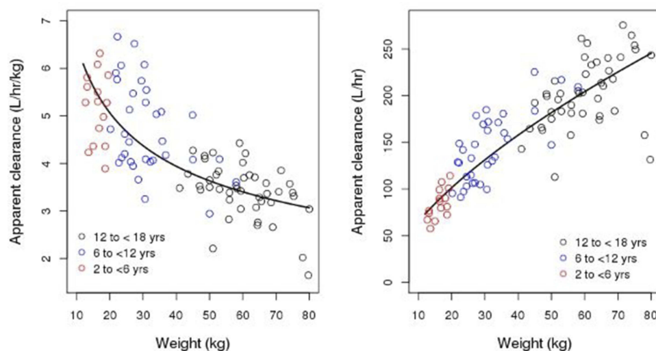
Figure 5 Empirical Bayesian estimates of bodyweight-normalized apparent clearance (left panel) and apparent clearance (right panel) versus weight together with modeled relationship, using a power function (line) (Table 2).
