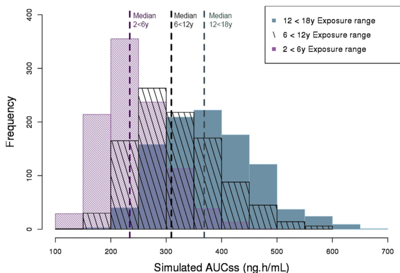
Figure S3 Overlaid histograms of the simulated AUCss produced following a dose of 1.25 mg/kg every 4 h in children aged 2 to <18 years. The median simulated AUCss for each age group are displayed.
