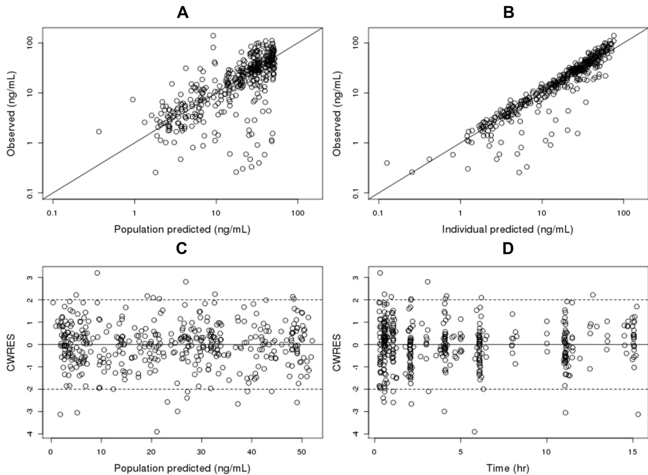
Figure 2 Plot of observed tapentadol concentration versus population predicted (A), observed tapentadol concentration versus individual predicted (B), conditional weighted residuals versus population predicted (C), conditional weighted residuals versus time (D). The black represents the identity line (A, B) or the zero line (C, D). Abbreviation: CWRES, conditional weighted residuals.
