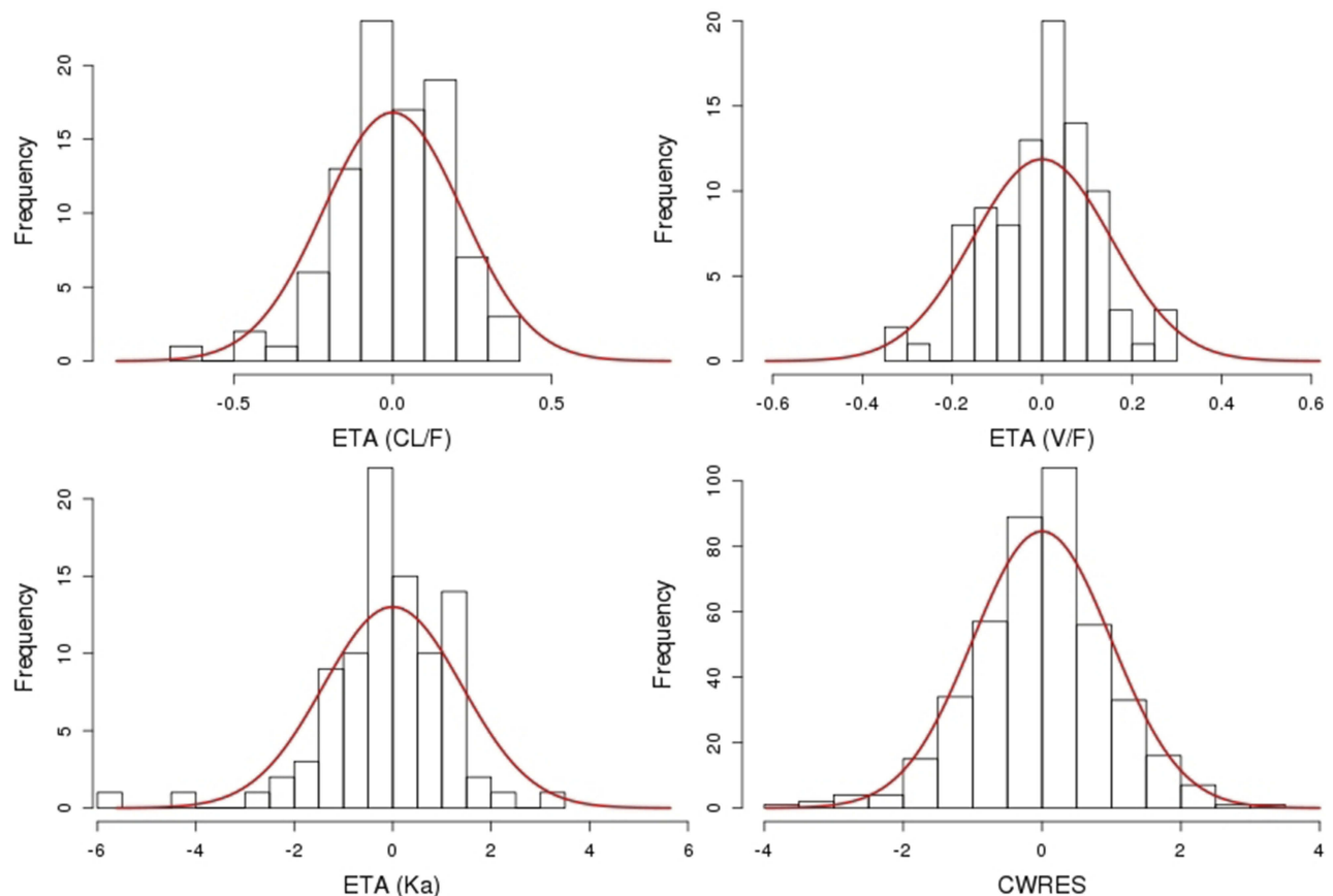
Figure S1 Histograms of the random effects (ETA) for clearance (CL/F), volume of distribution (V/F), absorption rate constant (Ka), and the conditional weighted residuals (CWRES). The solid line represents the scaled (by area) probability density functions with mean zero, and variances of ETA as estimated by mixed effects modeling (Table 2). The variance of CWRES is equal to one.
