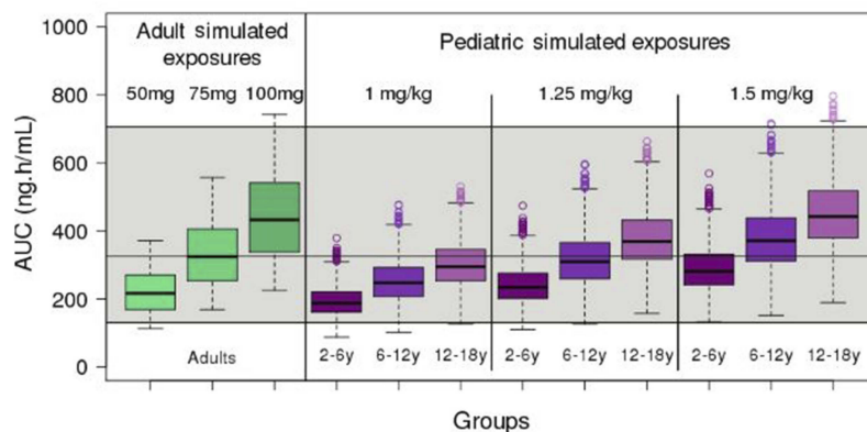
Figure 4 Boxplot of the simulated steady-state area under the curve (AUCss) of tapentadol in adults and pediatric subjects 2 to <18 years of age receiving 1.0 mg/kg, 1.25 mg/kg, and 1.5 mg/kg of tapentadol every 4 hrs. The gray shaded area represents the 2.5th and the 97.5th percentile of the AUCss in adults receiving 50 mg and 100 mg tapentadol every 4 hrs, respectively. The central black line indicates the 50th percentile (median) of the AUC in adults receiving 75 mg tapentadol every 4 hrs.
