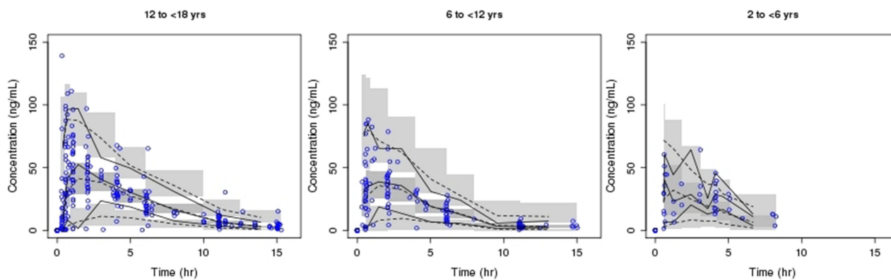
Figure S2 Simulation based visual predictive check (VPC) using final parameter estimates from the population pharmacokinetic model based on NCT01729728 and NCT01134536 data. Blue open circles represent observed tapentadol concentrations; solid lines represent observed 2.5th, median, and 97.5th percentile of tapentadol concentration-time course, dotted lines represent 2.5th, median, and 97.5th percentile of the predicted tapentadol concentration-time course; gray areas represent the corresponding 95% confidence intervals.
