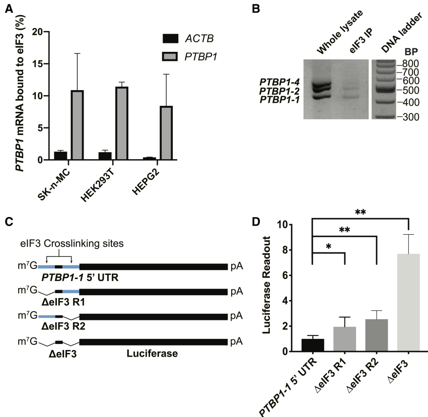
FIGURE 6. Binding of reporter mRNAs containing sites of interaction with eIF3. (A) qPCR quantification of PTBP1 mRNA bound to eIF3, with ACTB used as a negative control. Cell lines SK-n-MC, HEK293T, and HEPG2 were used. (B) PTBP1 mRNA exon 9 coding sequence isoforms that immunoprecipitate with eIF3, as determined by RT-PCR, and resolved on a 2% agarose. DNA ladder shown on the right. (C) Schematic of PTBP1 5'-UTR-luciferase reporter mRNAs. WT, wild-type; ΔeIF3, deletion of eIF3 PAR-CLIP clusters, nucleotide positions 25–49 (Region 1, R1), and/or 58–86 (Region 2, R2) for the PTBP1 transcript with the long 5'-UTR (GenBank accession NM_002819). (D) Luciferase activity in HEK293T cells transfected with mRNAs containing PTBP1 5'-UTR elements with or without deletions of the eIF3 crosslinking sites in Region 1 (R1) and/or Region 2 (R2). Experiments were carried out in biological triplicate, with standard deviation shown, significant with (*) P > 0.01 , (**) P > 0.001 .
