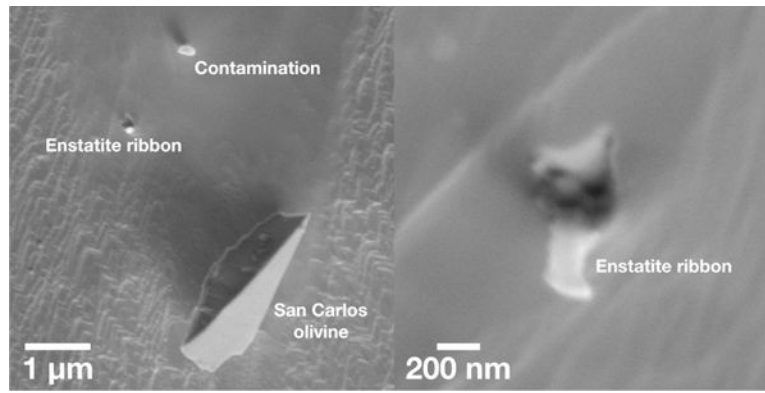
Figure 3: Enstatite ribbon mounted for O isotope analyses. The ribbon stuck to the Au mount nearly perpendicular to its surface.
