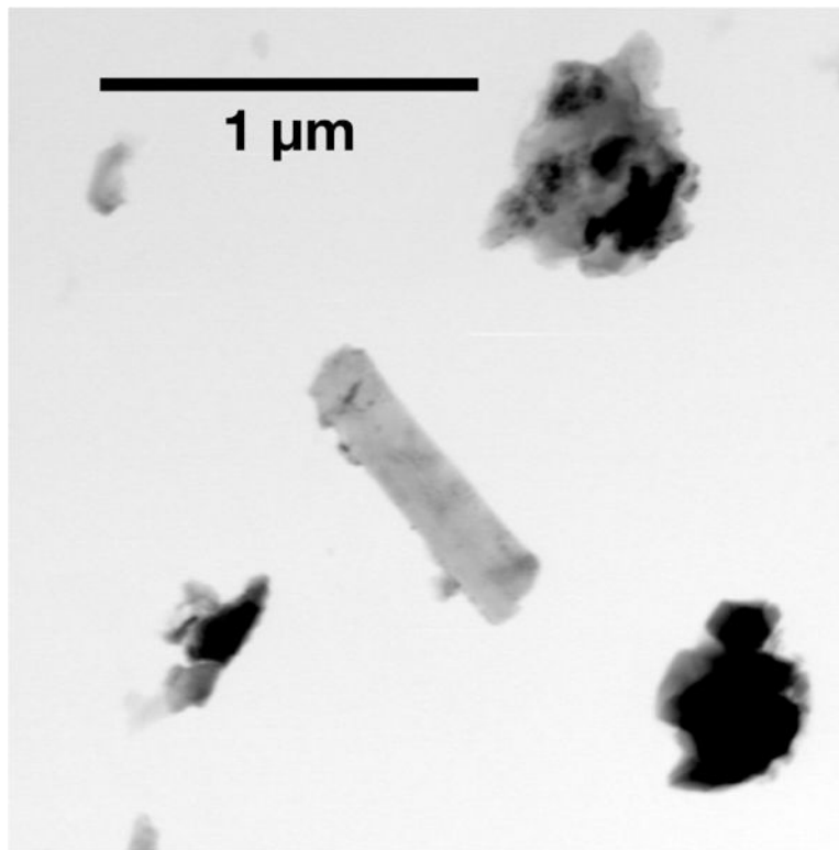
Figure 2: Bright-field TEM image of enstatite ribbon.
