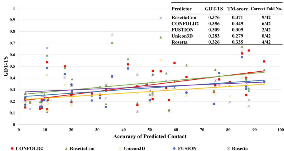
FIGURE 8 The modeling performance of contact-based ab initio modeling methods vs the predicted contact accuracy (L/5 contacts) in CASP13. Each point represents the modeling accuracy in terms of GDT-TS score vs the accuracy of predicted contacts for a method. The colors represent different modeling methods. Rosetta without contacts (purple) was included for comparison. The averaged GDT-TS score and TM-score of five methods on the all CASP13 targets are summarized in the top-right table
