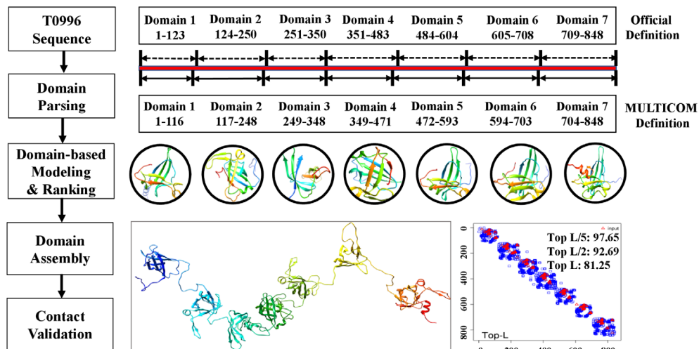
FIGURE 10 The successful modeling of a large multidomain target T0996 and the contact-based validation. The contacts (red) predicted by DNCON2 match with the contacts (blue) in the template-based models domain by domain
