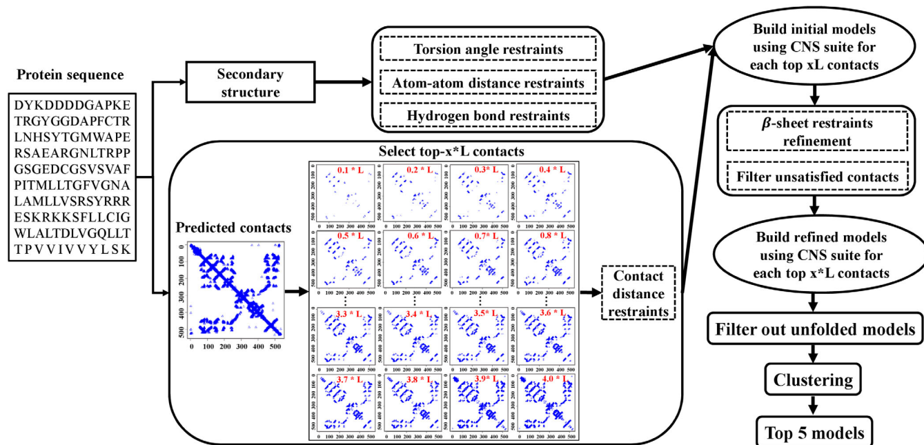
FIGURE 3 Automated contact distance-based ab initio protein structure prediction by CONFOLD2
