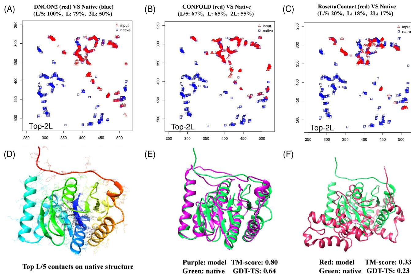
FIGURE 9 A successful ab initio modeling example (a domain of target T1000) for which no significant templates were identified. For the FM domain of T1000 (residues 282-523), the accuracy of top L/5 predicted contacts is 100%, top L 79% and top 2L 50%. CONFOLD2 successfully built a complicated \alpha -helix + \beta -sheet + \alpha -helix model for the domain with TM-score of 0.8 and GDT-TS of 0.64, while RosettaCon failed to generate a correct topology (ie, TM-score = 0.33 < 0.5 threshold). This example shows that the pure contact distance driven method such as CONFOLD2 can build high-quality structural models of complicated topology for large domains if a sufficient number of accurate contact predictions are provided
