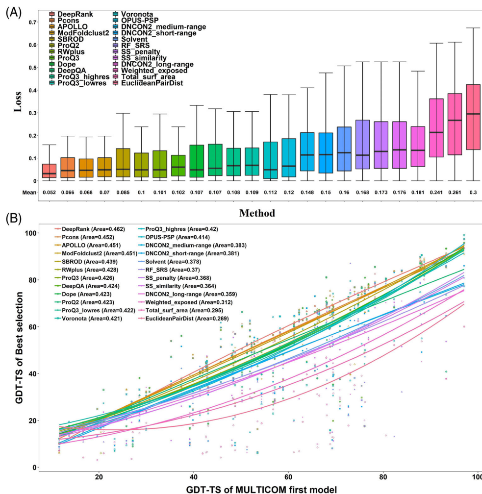
FIGURE 6 Comparison of DeepRank with individual QA methods used in MULTICOM predictors. A, The box plot of loss of each method. Here the loss is measure at 1-point scale (ie, the highest/perfect GDT-TS score = 1). B, The GDT-TS score at the 100-point scale of the top models selected by each individual QA method and DeepRank is plotted against the GDT-TS score of MULTICOM’s first submitted models for 74 “all group” full-length targets. The curve for each method is fitted by the second-degree polynomial regression function. The area under the curve for each method is calculated and shown on the top left. The larger area indicates the better capacity of model selection
