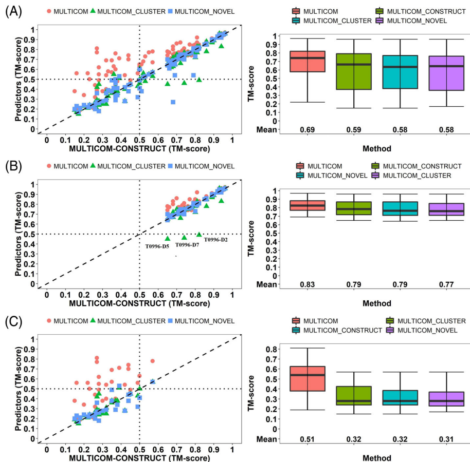
FIGURE 5 Evaluation of four MULTICOM predictors. The methods are ranked by average TM-score of the first (ie, TS1) submitted models. A, On 104 domains (left plot: TM_scores of MULTICOM, MULTICOM_CLUSTER, MULTICOM-NOVEL models vs TM_scores of MULTICOM-CONSTRUCT models; right plot: mean and variation of the TM-scores of the models of the four methods). B, On 40 template-based (TBM-easy) domains. C, On 31 template-free (FM) domains
