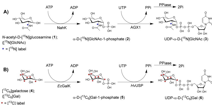
Scheme 1. Repetitive batch synthesis for (A) isotope-labeled UDP-[ ^{15}\text{N} ]GlcNAc (3) by the N -acetylhexosamine-1-kinase (NahK), UDP-GlcNAc pyrophosphorylase (AGX1), and an inorganic pyrophosphatase (PPIase) and (B) isotope-enriched UDP-[ ^{13}\text{C}_6 ]Gal (6) by galactokinase ( EcGalK ), the UDP-sugar pyrophosphorylase from Hordeum vulgare ( HvUSP ) and PPIase.
