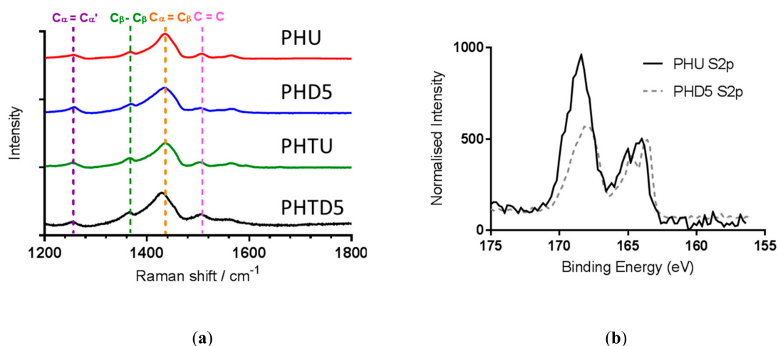
Figure 5. (a) Raman spectra for Clevios fibers untreated and treated with DMSO for 5 min. Untreated and 5 min DMSO treatments for PH1000 thick and PH1000 thin. (b) XPS spectra showing S2p emission for fibers PHU and PHD5.
