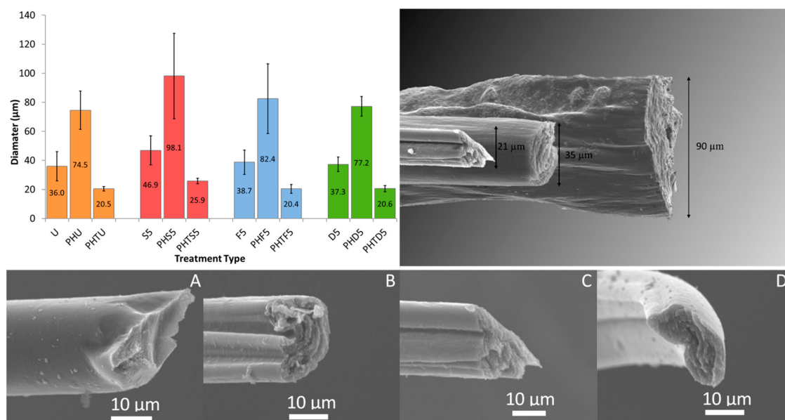
Figure 3. Averaged diameter values comparing Orgacon PEDOT:PSS fibers with both diameters of Clevios PH1000 fibers for 5 min treatments ( top left ) ( n = 10 ). SEM graphic comparing the three fiber types ( top right ). SEM images of fiber cross-sections PHTU ( A ), PHTS5 ( B ), PHTF5 ( C ), PHTD5 ( D ).
