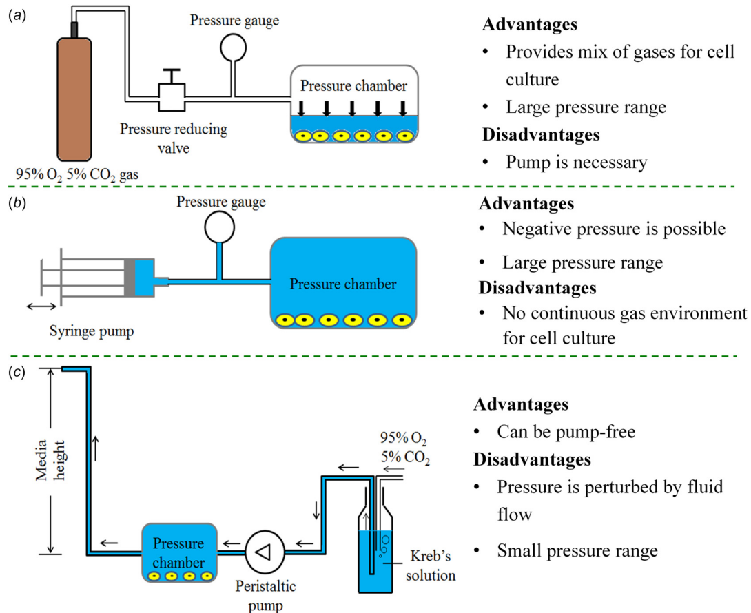
Fig. 2 Existing approaches for altering hydrostatic pressure in the cell micro-environment: (a) the gas pressure method [25,75], (b) the syringe method [44,76], and (c) the media height method [77,78]
