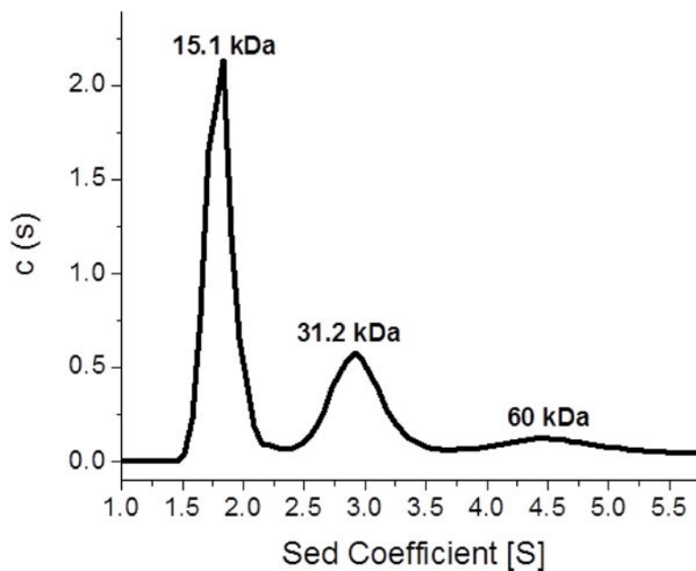
Figure 3. AUC for the determination of the oligomeric states of apo human BOLA3, monitored at 280 nm. The first peak of the black trace at 15.1 kDa accounts for 54% of the sample, the second peak at 31.2 kDa accounts for 30%, and the third peak at 60 kDa corresponds to 14% of the sample. The AUC results were obtained by fitting the sedimentation data to the Lamm equation [3, 4] using a continuous distribution model.
