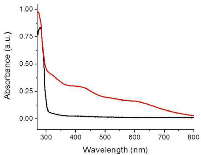
Figure 1. UV spectra of apo BOLA3 (black) and holo BOLA3 reconstituted using ferric chloride, L-cysteine and Tm NifS (red). Charge-transfer bands indicative of a bound Fe-S cluster are present at 330 and 420 nm.
