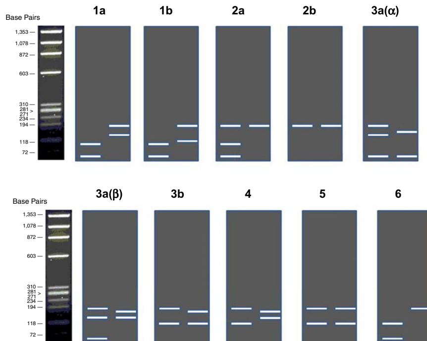
Fig. 2. Diagrammatic representation of the digestion pattern of 5'NCR PCR-RFLP.
