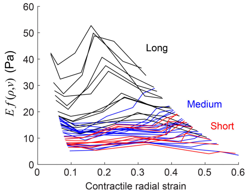
Figure 9: Product of Young's modulus E and function f(v, \rho) measured by particles in collagen networks having short (red), medium (blue), or long (black) fibers. Each line represents a measurement by a different PNIPAAm particle. The horizontal axis gives contractile strain of each particle, which is equal to the magnitudes of normal strains within the collagen network at each particle–network interface.
