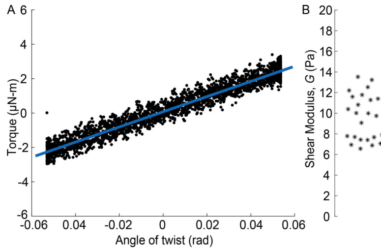
Figure 4: Shear modulus of polyacrylamide. (A) Torque plotted versus angle of twist for one polyacrylamide specimen. From the linear fit and the specimen's dimensions, the shear modulus was computed. (B) Shear modulus measured for 24 different polyacrylamide gels.
