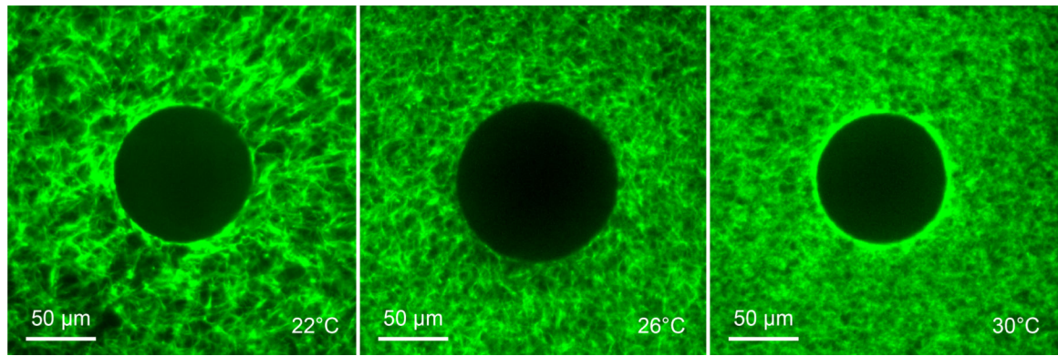
Figure 5: Collagen networks (3 mg/ml) polymerized at 22°C, 26°C and 30°C having long, medium, and short fibers, respectively.
