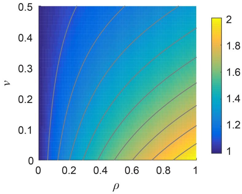
Figure 1: Dimensionless function f(\nu, \rho) defined in Eq. 9, where \nu is Poisson's ratio and \rho is the dimensionless compression weakening factor. Contour lines show values of f = 1.1, 1.2, \dots, 1.9 .
