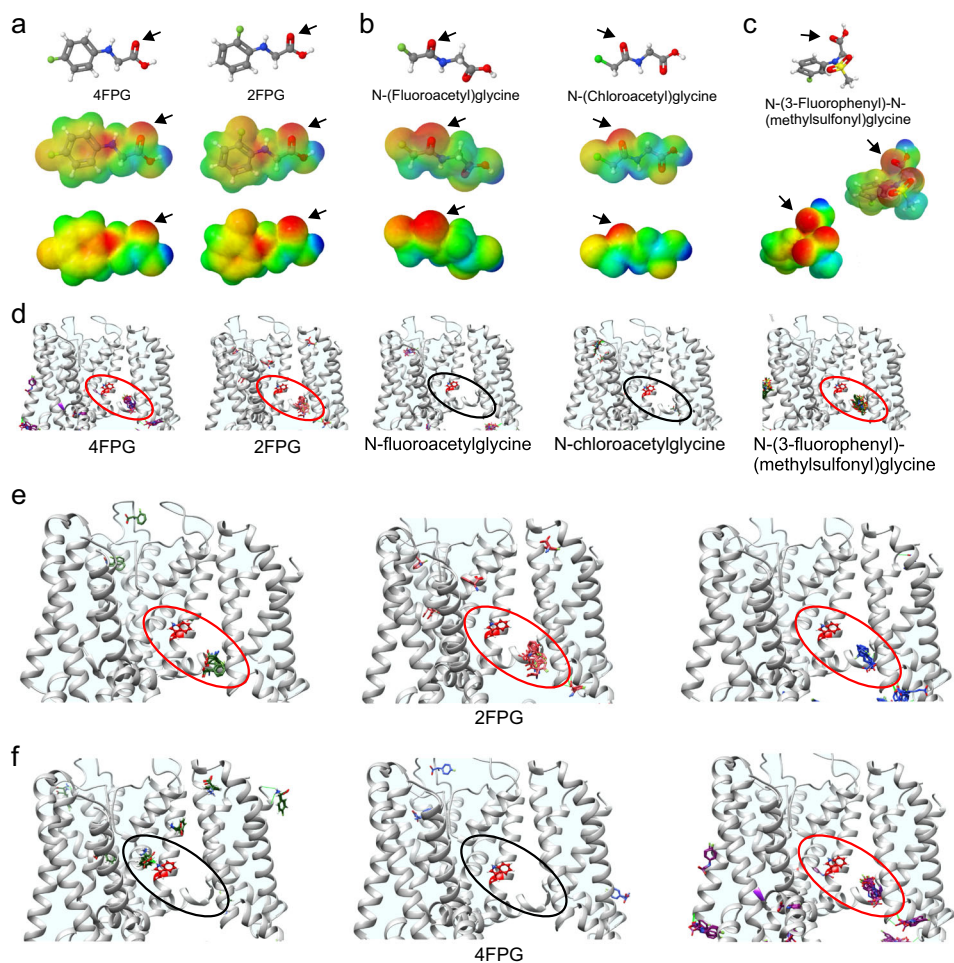
Fig. 3 In silico prediction of 4FPG-related KCNQ-activating glycine derivatives. a Chemical properties of 4FPG versus 2FPG: structure, electrostatic surface potentials (red, electron-dense; blue, electron-poor; green, neutral) and an overlay of the two, all calculated and plotted using Jmol. Arrows, native glycine carbonyl. b, c Chemical properties of 4FPG-related glycine derivatives, parameters as in (a). Arrows, non-native glycine carbonyls for N-(fluoroacetyl)glycine and N-(chloroacetyl)glycine; native glycine carbonyl for 3FMSG. d Docking results showing predicted binding (red ovals) or lack thereof (black ovals) of the compounds in (a-c) to the GABA binding pocket in the KCNQ1/KCNQ3 structural model. Red side-chain, KCNQ3-W265. e Docking results showing predicted binding (red ovals) of three different conformational forms of 2FPG to the GABA binding pocket in the KCNQ1/KCNQ3 structural model. Red side-chain, KCNQ3-W265. f Docking results showing predicted binding (red oval) or lack thereof (black ovals) of three different conformational forms of 4FPG to the GABA binding pocket in the KCNQ1/KCNQ3 structural model. Red side-chain, KCNQ3-W265
