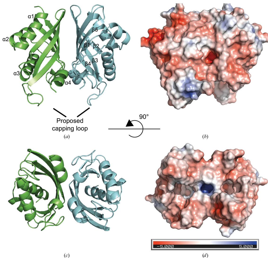
Figure 2 The structure of IdmH. (a, c) Ribbon diagrams showing the IdmH dimer architecture. Individual monomers are coloured green and blue, respectively. The overall shape of the monomer can be described as a distorted \alpha/\beta -barrel with the dimerization interface located between the \beta -sheets. Each monomer comprises four \alpha -helices ( \alpha 1– \alpha 4) and five \beta -strands ( \beta 1– \beta 5). (b, d) Surface representation of the IdmH dimer. The surface is coloured using APBS (Jurrus et al. , 2018) according to the approximate electrostatic potential from -5 \text{ kT e}^{-1} (red) to 5 \text{ kT e}^{-1} (blue).
