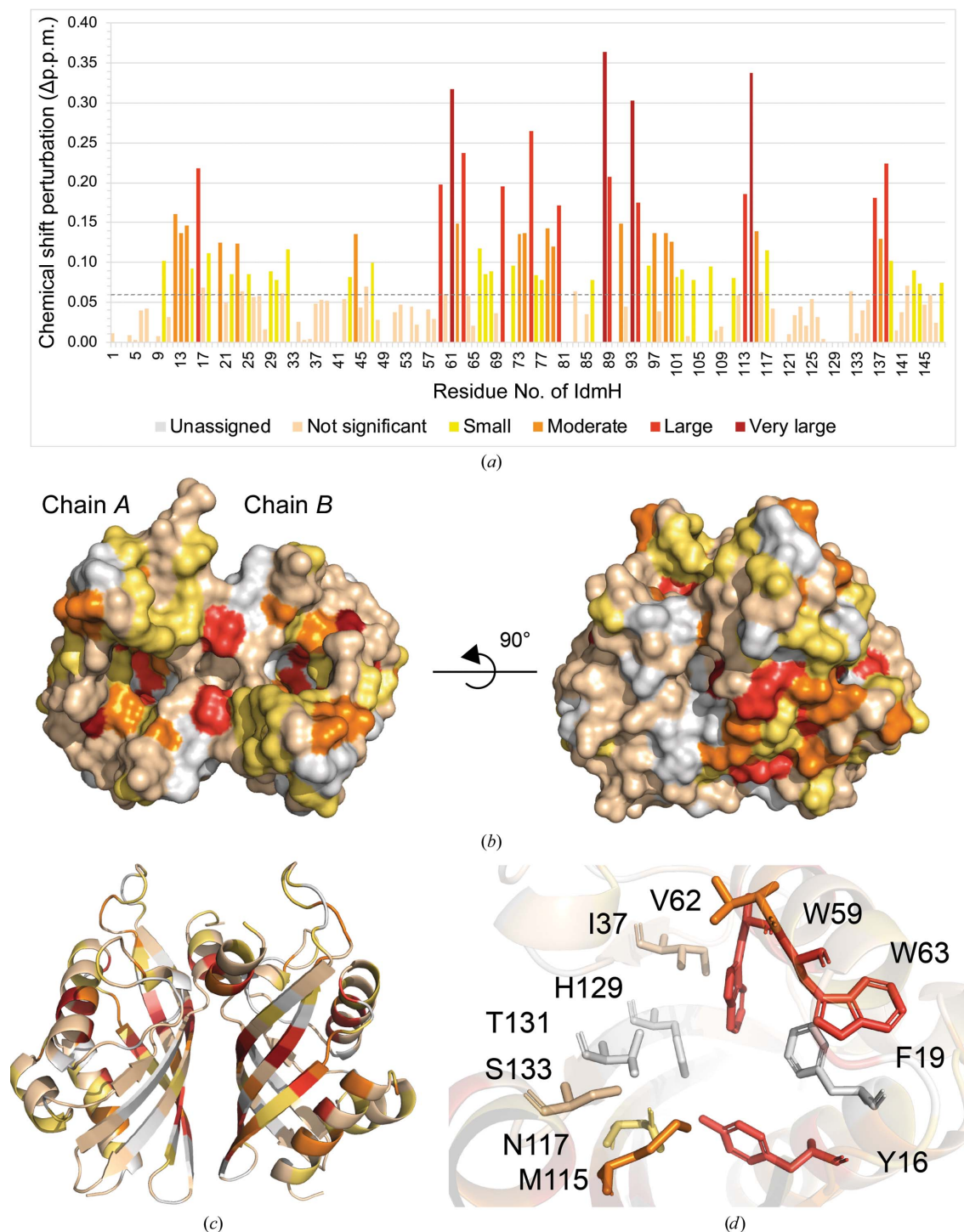
Figure 6 Chemical shift perturbations (CSPs) mapped onto IdmH following the addition of indanomycin. (a) Histogram showing the geometrical distance moved by each peak assigned to a residue. Peaks are coloured from yellow to dark red as the value of the CSP increases. Chemical shifts which were smaller than the standard deviation of all shifts (0.072 p.p.m.) are coloured pale cream. Surface (b) and ribbon (c) representations of IdmH with peak shifts mapped using the same colour scheme as in (a). Residues which could not be assigned in the NMR spectrum are coloured white. (d) Active-site cavity of chain B with the proposed catalytic residues coloured according to the same colour scheme as in (b) and (c).
