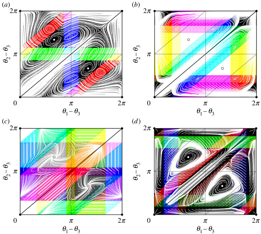
Figure 8. The phase space for (1.2) with N = 3 oscillators and coupling function g with one dead zone as in (5.2) and parameters as in figure 7a–d respectively. As in figures 5 and 6, black lines indicate the sets \theta_1 - \theta_2 = 0 , \theta_2 - \theta_3 = 0 and \theta_3 - \theta_1 = 0 which intersect in \Theta^{\text{sync}} (black dot, \bullet ) that bound \mathcal{C} and its symmetric image. The splay phases are indicated by hollow dots ( \circ ) and dashed lines indicate phase configurations where one phase difference is equal to \pi . As above, the colouring indicates the effective coupling graph overlaid by trajectories started on a regular grid, shown in white—a very wide range of effective coupling graphs are realised; see figure 9. For (b) and (c), there are white regions of trivial dynamics where no trajectories are present: these correspond to the effective coupling graph \emptyset_3 . Finally, note that for (a) and (c) there are trajectories that visit \Theta_g(\mathbf{H}) for multiple \mathbf{H} \in \mathcal{H}_3 as time evolves. (Online version in colour.)
