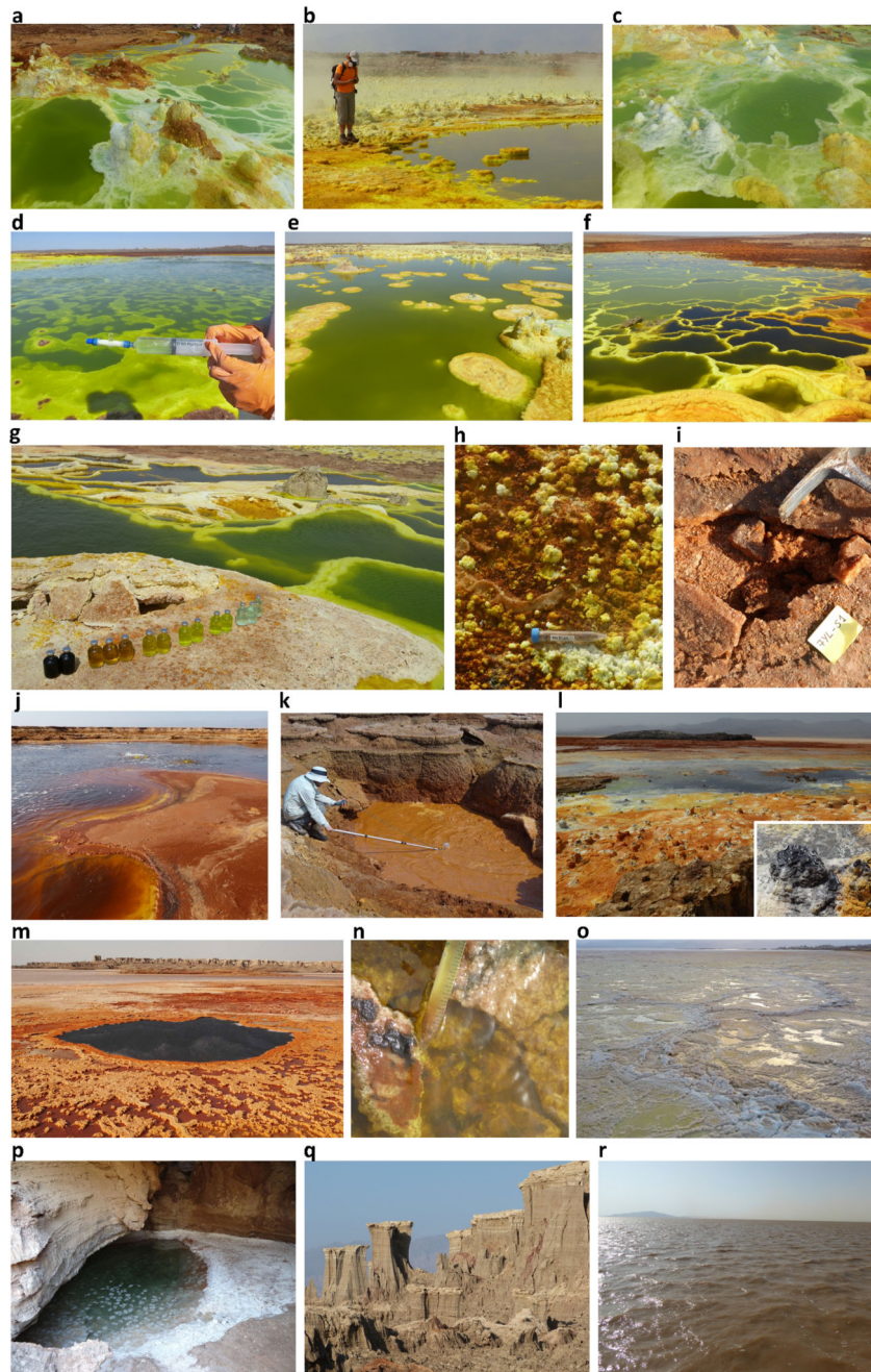
Extended Data Fig. 2. Views of different sampling sites in the Dallol dome and surroundings in the Danakil Depression.
