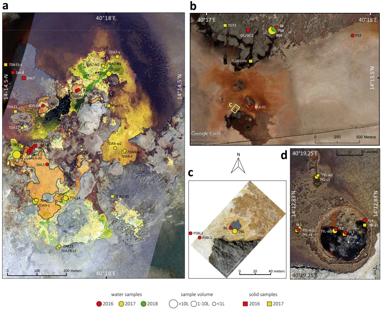
Extended Data Fig. 1. Aerial view of the main sampling sites in the Dallol area.
