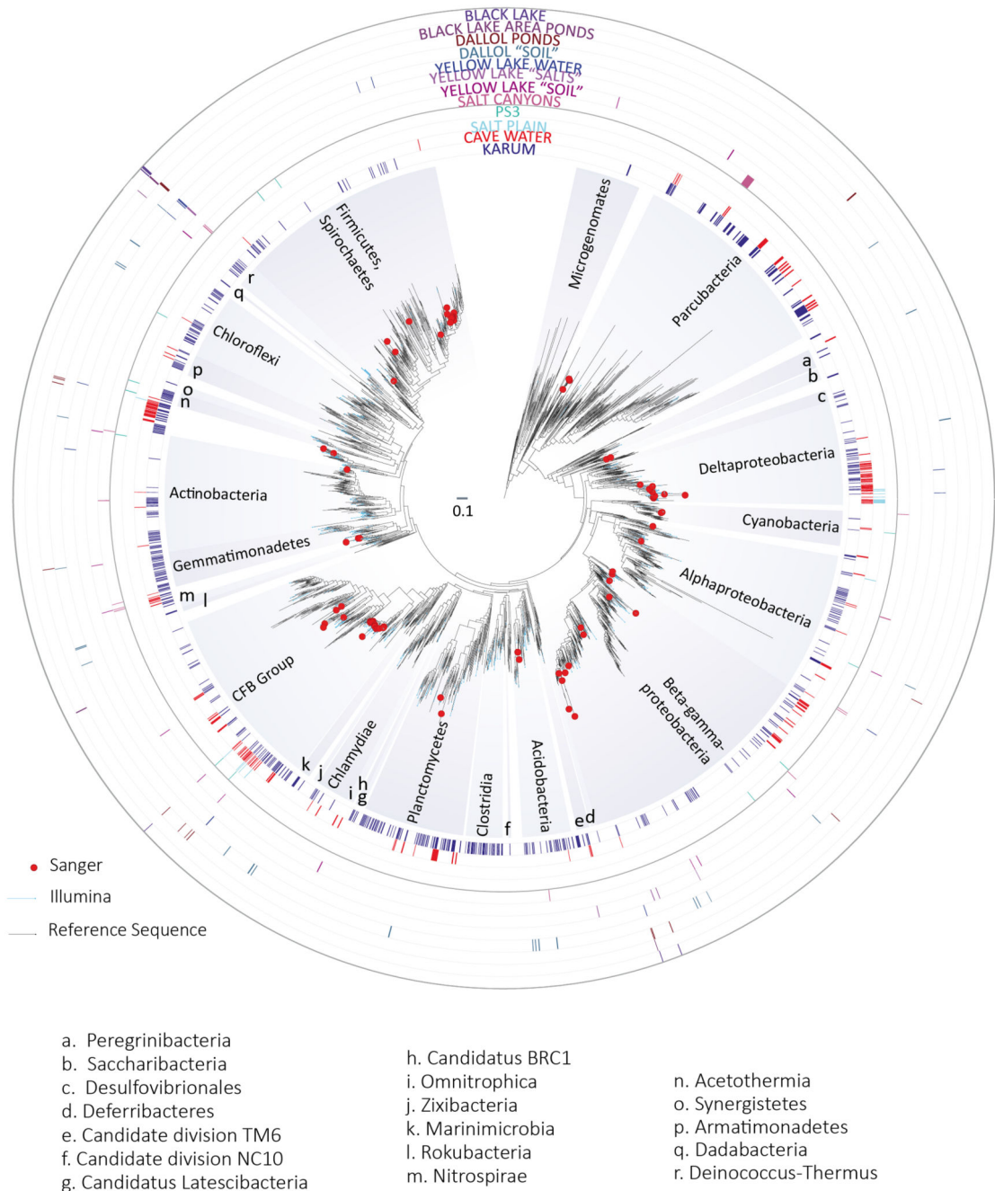
Extended Data Fig. 7. Phylogenetic tree of bacterial 16S rRNA gene sequences showing the phylogenetic placement of OTUs identified in the different Dallol area samples.
