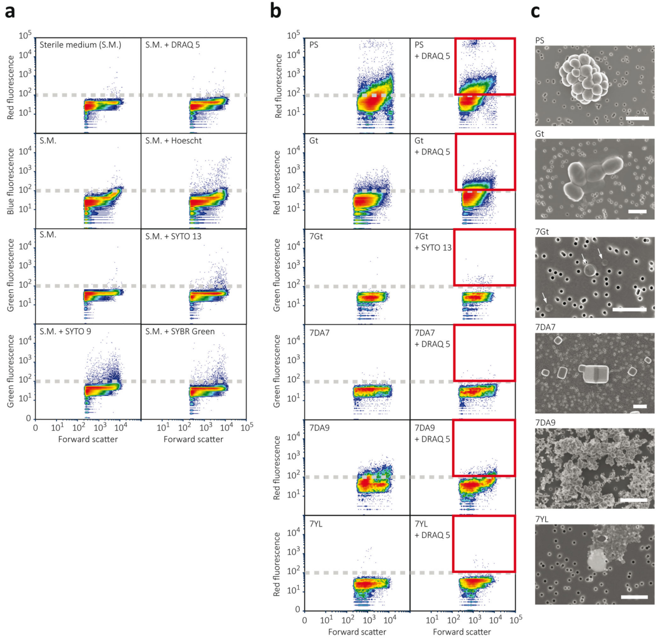
Extended Data Fig. 9. Multiparametric fluorescence analyses and fluorescence-activated cell sorting (FACS) analyses of representative Dallol area samples.
