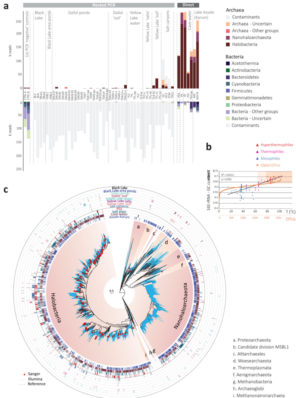
Fig. 3. Distribution and diversity of prokaryotes in samples from the Dallol mound and surrounding areas based on 16S rRNA gene metabarcoding data.
