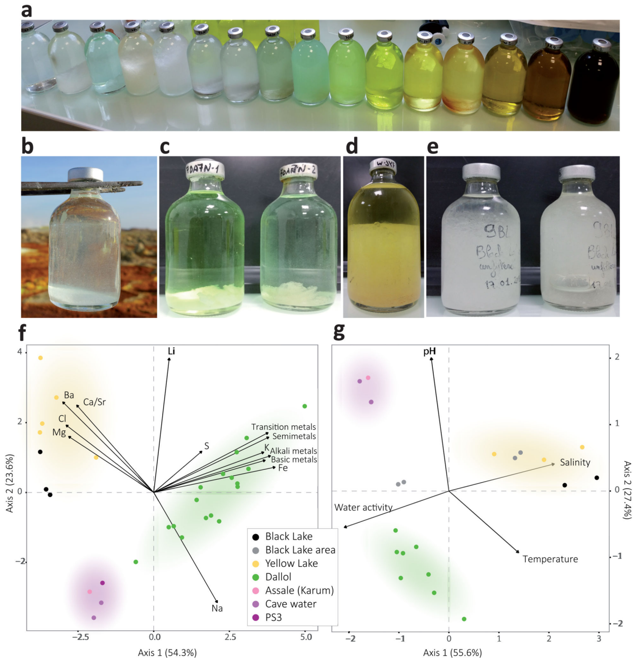
Fig. 2. Physicochemical features of liquid samples from the Dallol area.
