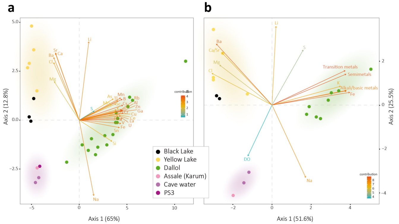
Extended Data Fig. 4. Principal Component Analyses (PCA) of Dallol area sampling sites as a function of physicochemical parameters.
