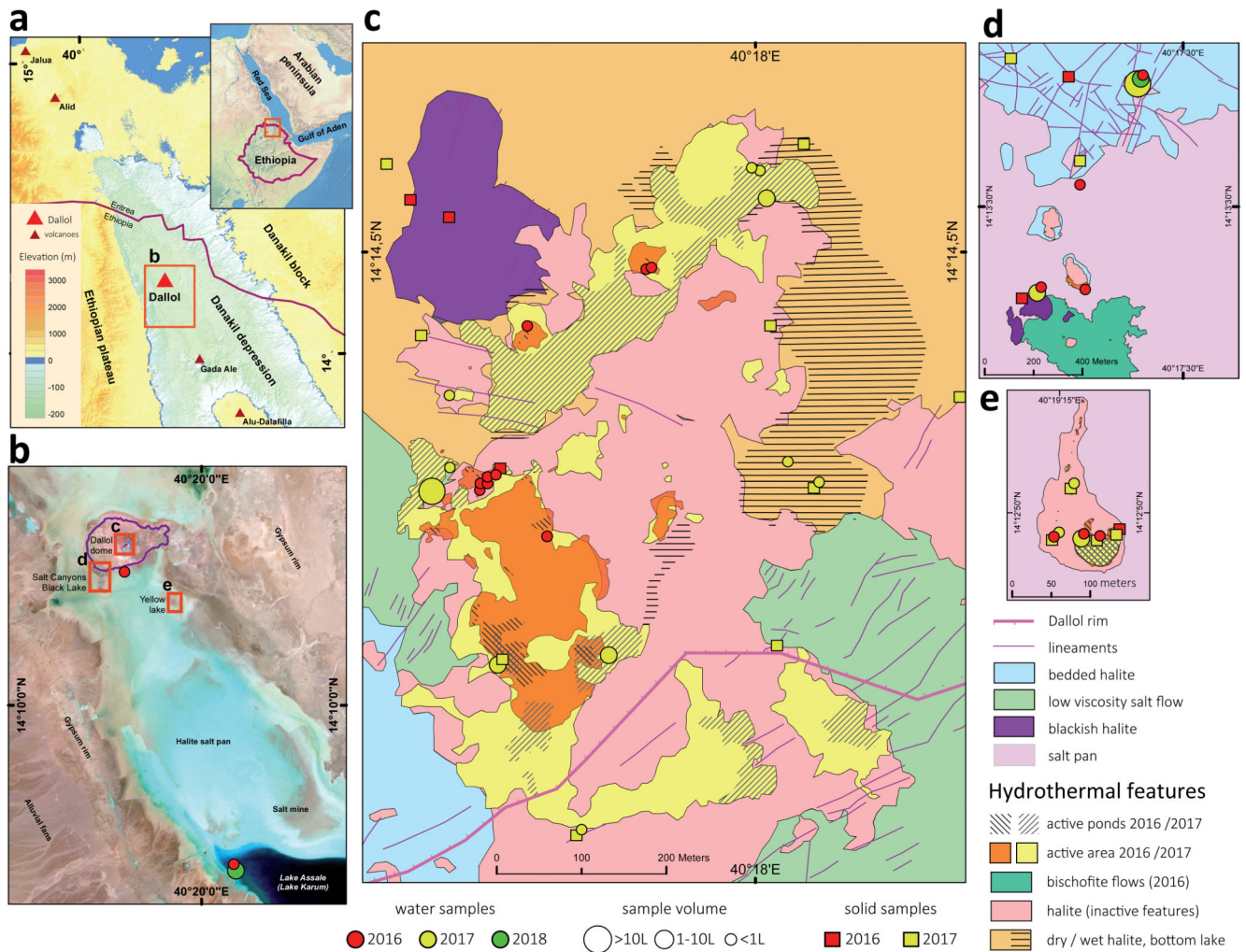
Fig. 1. Overview of sampling sites at the polyextreme geothermal field of Dallol and its surroundings in the Danakil Depression, Ethiopia. a , Location of the Dallol dome area in the Danakil Depression following the alignment of the Erta Ale volcanic range (Gada Ale, Alu-Dalafilla), Northern Ethiopia; b , closer view of the sampling zones in the Dallol area and Lake Assale or Karum (satellite image from Copernicus Sentinel 1; 2017, January 19th); c-e , geological maps showing the sampling sites at (c) the Dallol dome summit, (d) West salt canyons and Black Mountain, including the Black Lake and (e) Yellow Lake (Gaet' Ale) zone. Squares and circles indicate the nature of collected samples and their color, the collection date. The size of circles is proportional to the collected brine volume for analyses. Specific sample names are indicated in the aerial view shown in Extended Data Fig. 1.
