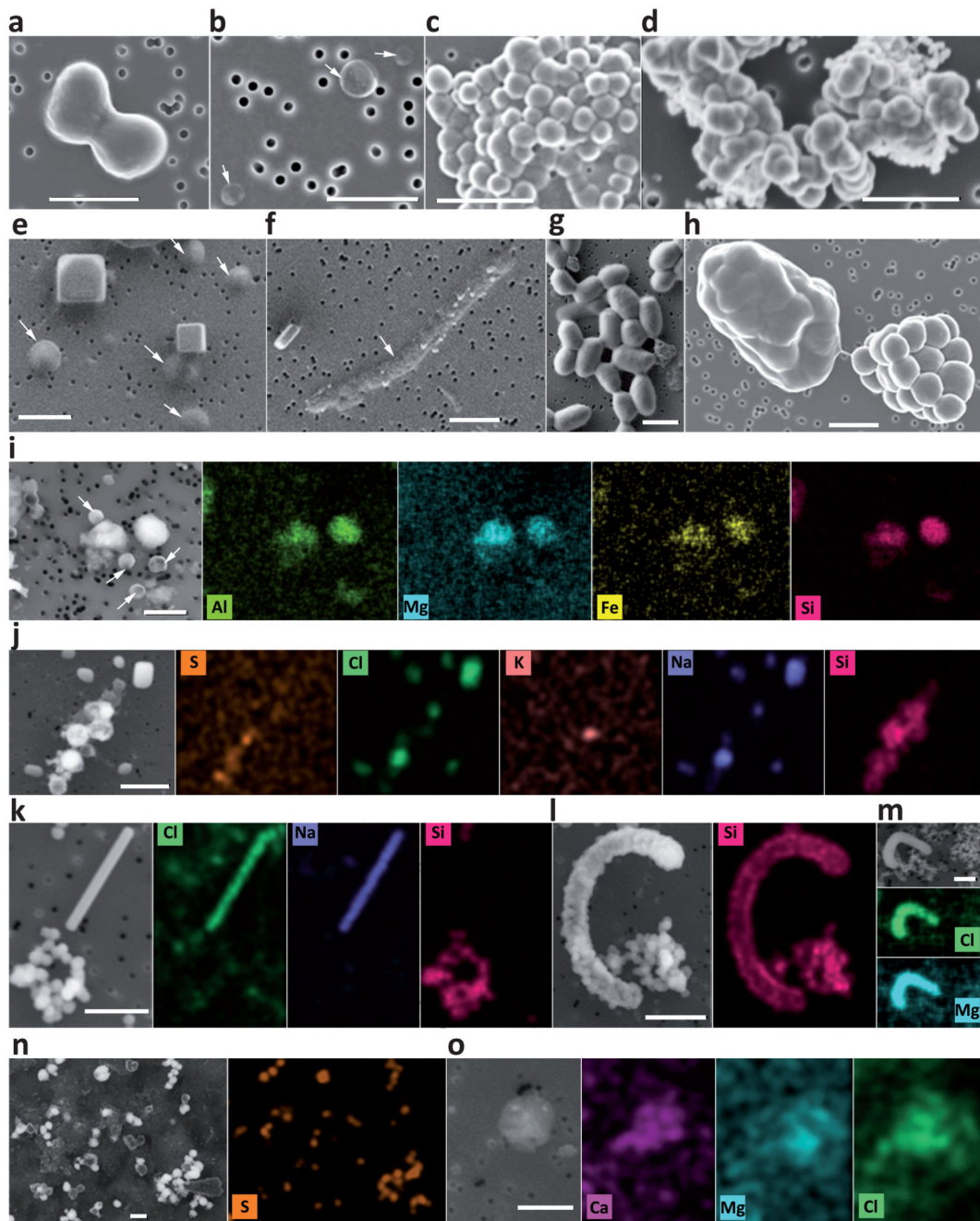
Fig. 4. Scanning electron microscopy (SEM) pictures and chemical maps of cells and abiotic biomorphs identified in samples from the Dallol region.
