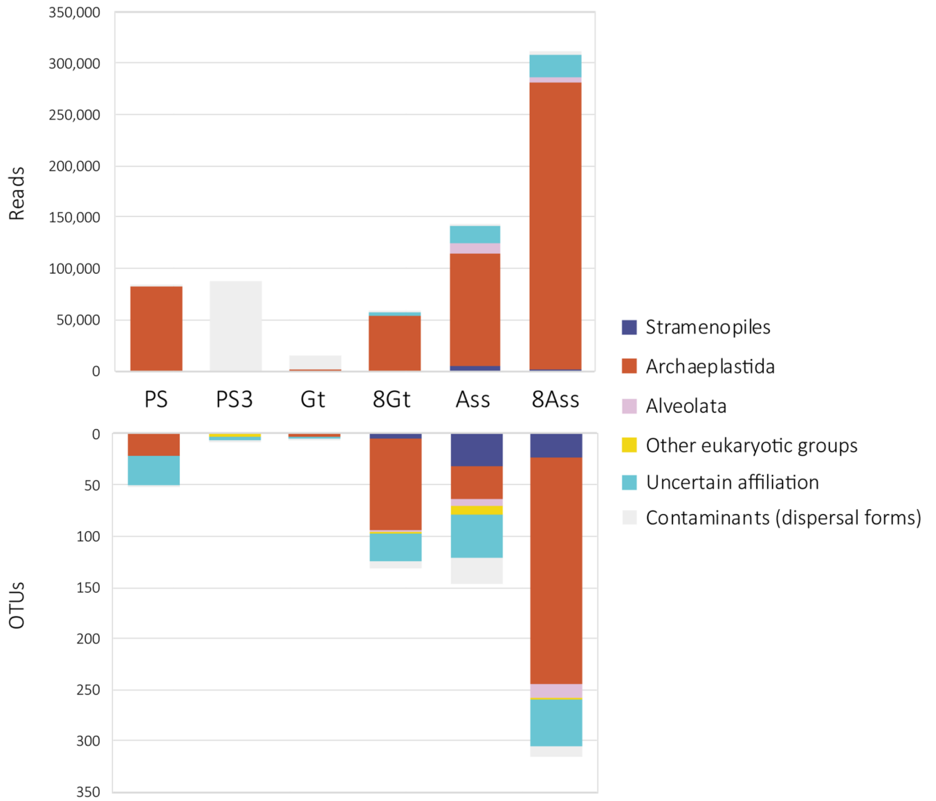
Extended Data Fig. 8. Eukaryotic presence, diversity and relative abundance in Dallol area samples.
