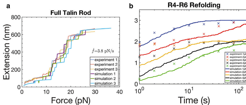
FIGURE 9 ( a ) Unfolding of a full talin rod compared to the experimental measurements of Yao et al. (69,70); unfolding as observed under imposed force rate. ( b ) Talin domain refolding is shown. To see this figure in color, go online.
