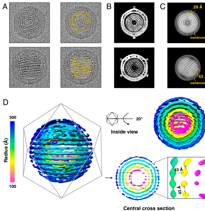
Fig. 3. Asymmetrical reconstruction of SPV1. (A) Two distinctive views of SPV1 from the raw EMs, showing concentric rings ( Top ) and striations ( Bottom ). (B) The central portion of the asymmetrical reconstruction of SPV1 filtered to 40 Å in the corresponding orientations shown in A. (C) Two-dimensional class averages of masked SPV1 (excluding the outer capsid) match both views seen in A. In the Top average, there is a strong helical periodicity along the nucleoprotein filaments with a pitch of 29 Å. In the Bottom average, the 43-Å spacing between layers is evident. (D) The same EM map in B showing the genome region only, colored by radius. A central section ( Bottom Right ) highlights the conserved 43-Å spacing between layers and between filaments in the same layer.
