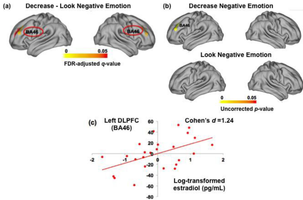
Figure 2. Relationships between estradiol levels and DLPFC activity during down-regulation of negative emotion
