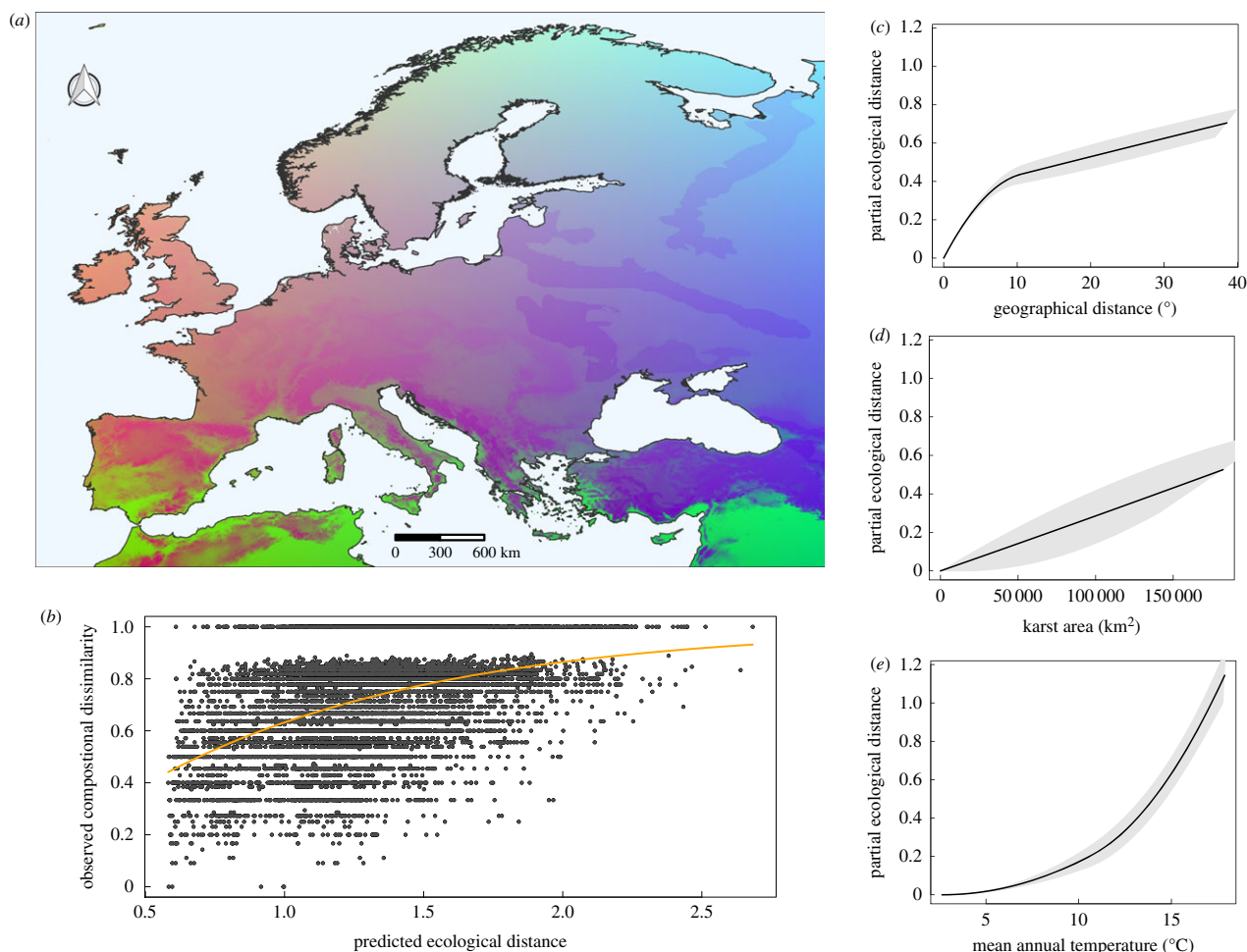
Figure 3. Results of generalized dissimilarity model for troglophile spider communities across Europe. (a) Predicted spatial variation in troglophile spider community composition. Colours represent gradients in species composition derived from transformed environmental predictors, whereby areas with similar colours are expected to contain more similar communities. (b) Relationship between observed compositional dissimilarity in troglophile spider community between each cave pair and the linear predictor of the regression equation from generalized dissimilarity model. (c–e) Fitted l-splines (partial regression fits) for variables significantly associated with \beta -diversity of troglophile spiders. The maximum height reached by each curve indicates the total amount of compositional turnover explained by that variable (holding all other variables constant), whereas the shape of each spline indicates how the rate of compositional turnover varies along the environmental gradient. (Online version in colour.)
