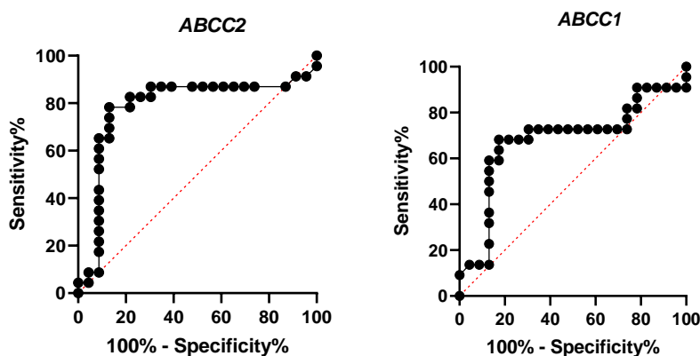
Fig. 2. ROC curves of ABCC1 and ABCC2 expression for evaluation of sensitivity and specificity in patients:
