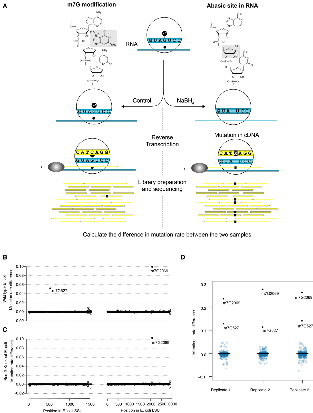
Figure 1. (A) Schematic representation of the m7G-MaP-Seq method. NaBH 4 treatment leads to formation of abasic sites at m7G positions, which subsequently are converted into cDNA mutations during reverse transcription and detected by massive parallel sequencing. (B) Detection of m7G at E. coli SSU rRNA position 527 and E. coli LSU rRNA position 2069 in WT strain. (C) Detection of m7G at E. coli SSU rRNA position 527 and E. coli LSU rRNA position 2069 in RsmG knockout strain. (D) Boxplots showing consistent detection of m7G modified positions in biological replicates.
