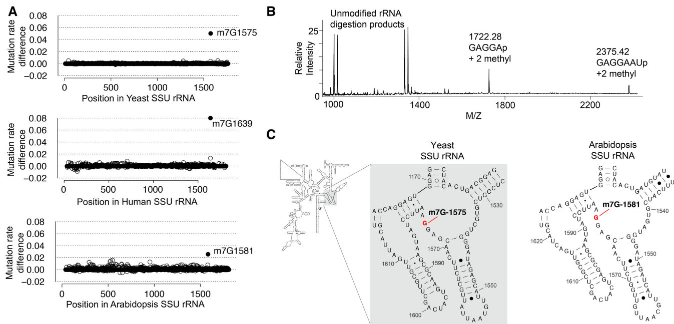
Figure 2. (A) Detection of m 7 G modifications in yeast, human and arabidopsis SSU rRNA. (B) Detection and validation of the m 7 G modification at Arabidopsis SSU rRNA position 1581 using mass spectroscopy. (C) Conservation of SSU rRNA m 7 G modification between yeast and Arabidopsis (secondary structures from the CRW database).
