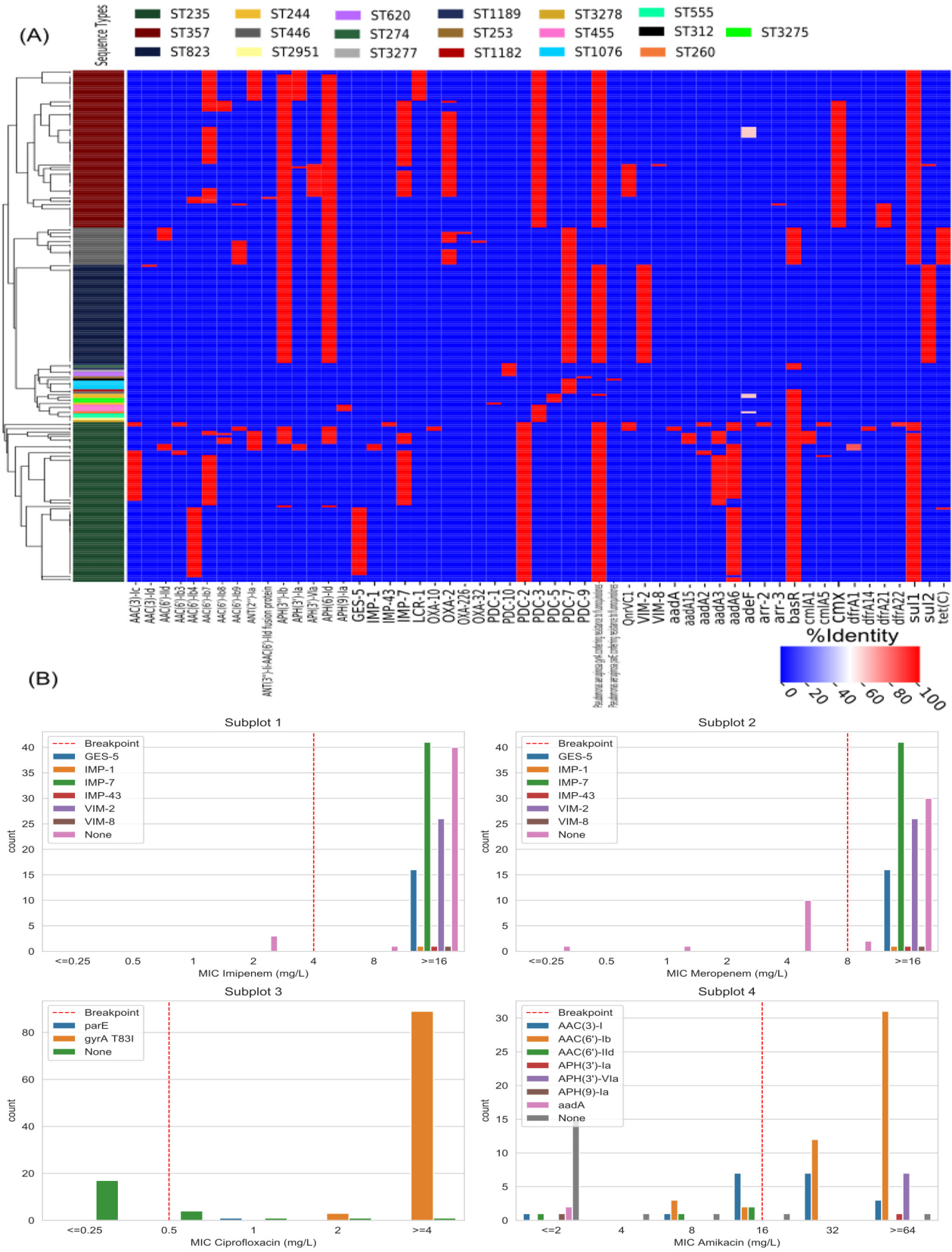
FIG 2 (A) Antimicrobial resistance heat map of 130 isolates of carbapenem-nonsusceptible P. aeruginosa (CNPA). The x axis contains only AMR determinants that were variably present in the CNPA collection. The following AMR determinants are not displayed because they were present in all (Continued on next page)
