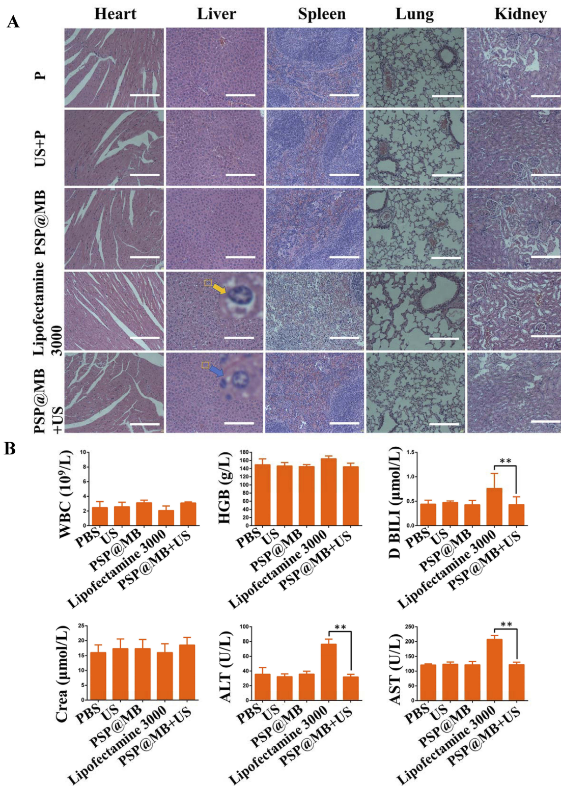
Figure 7 Biosafety evaluation.
