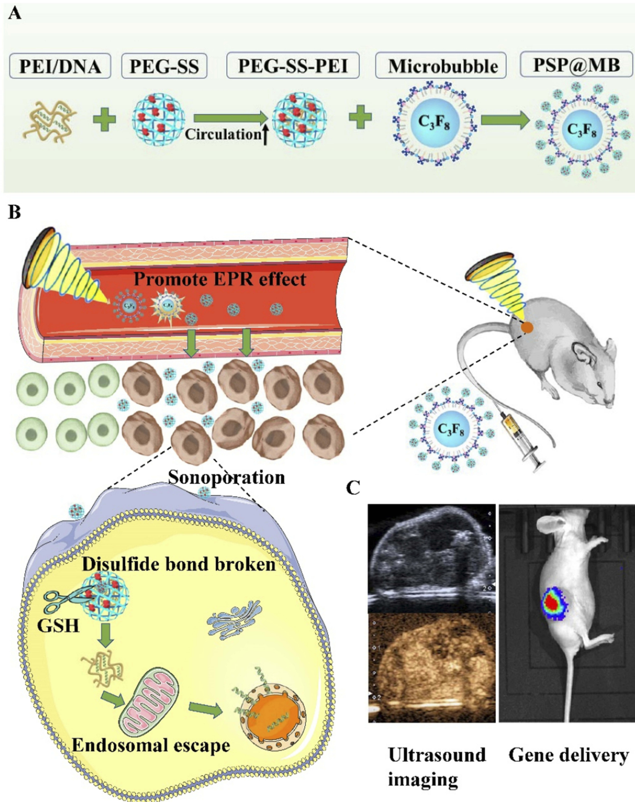
Figure 1 Graphical abstract.
