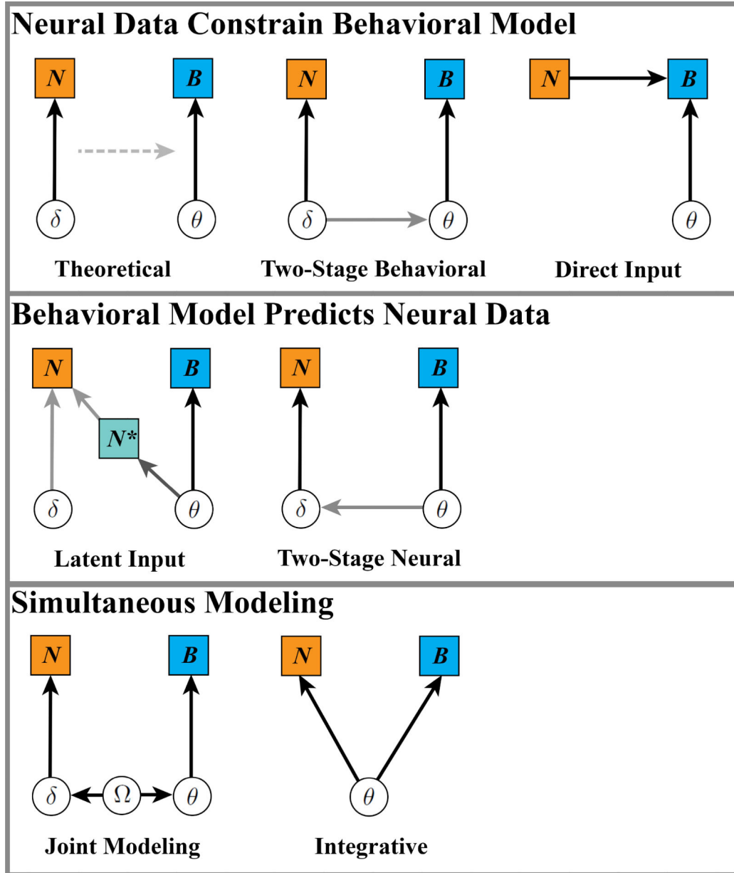
Figure 1: An illustration of several approaches used for linking neural and behavioral data, organized by specific modeling goals. N represents the neural data, B represents the behavioral data, N^* represents simulated internal model states, and \theta , \delta , and \Omega represent model parameters. When an approach is procedural, progression through processing stages is represented by arrows of decreasing darkness (e.g., the Latent Input Approach). Dashed lines indicate conceptual constraints (e.g., the Theoretical Approach), whereas solid lines indicate statistical constraints.
