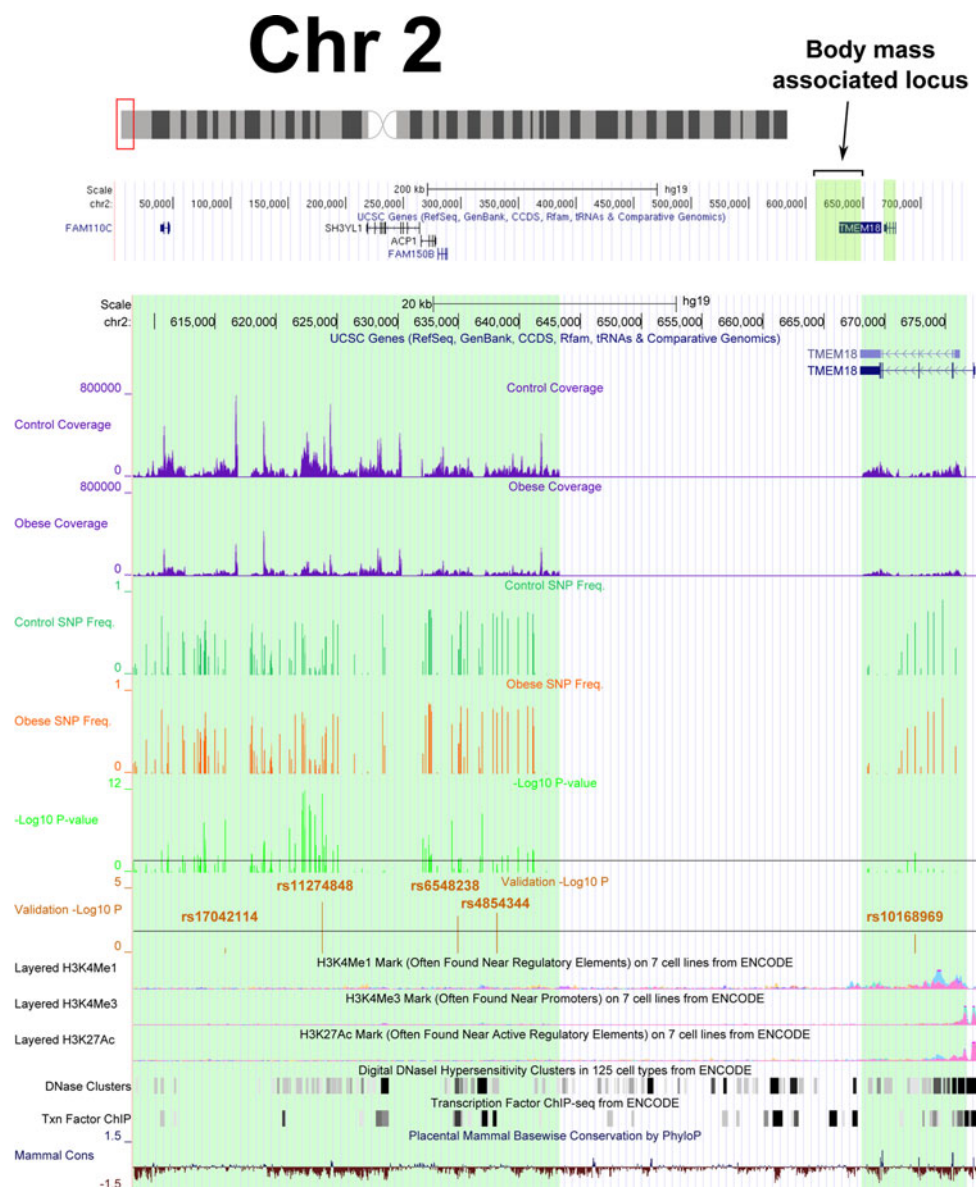
Fig. 1. Graphical representation of the location of TMEM18 on chromosome 2p25.3. Resequenced regions are highlighted in green. Coverage was measured as the number of reads mapped to each site achieved during re-sequencing of the obese and control DNA pools. Allelic frequencies of the alternative (non-reference allele) for all genetic variants detected during the re-sequencing in the control (green) and obese (orange) DNA pools are shown. Associations with obesity and odds ratios were determined by applying the Chi squared test. Negative log 10 p-values are displayed. 57 SNPs were identified after adjusting for multiple testing with the FDR. p-values < 0.023 were considered significant, represented here by the black line. A total of 55 SNPs present in the TMEM18-linked haplotype block, were identified as candidate SNPs for association with obesity. Additional information was gathered from the ENCODE project and integrated with the sequencing data. Markers for functional genomic elements included modifications of histone 3: mono-methylation of lysine 4 (H3K4Me1), tri-methylation of lysine 4 (H3K4Me3), as well as acetylation of lysine 27 (H3K27Ac); indicating transcription enhancer sites. Different cell lines are represented in different colours (additional information can be obtained via the UCSC website at http://genome.ucsc.edu/ ). DNase hypersensitivity regions, usually related to accessible chromatin, were included. Also included are transcription factor binding sites obtained from ChIP-seq. Darker colouration corresponds to stronger signal for possible binding sites. Conservation in vertebrate species for each base pair in the genomic sequence is included (Mammal Cons).
