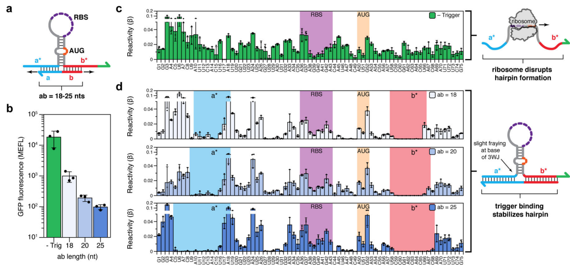
Figure 3 | In-cell SHAPE-Seq confirmation of the 3WJ repressor mechanism.
