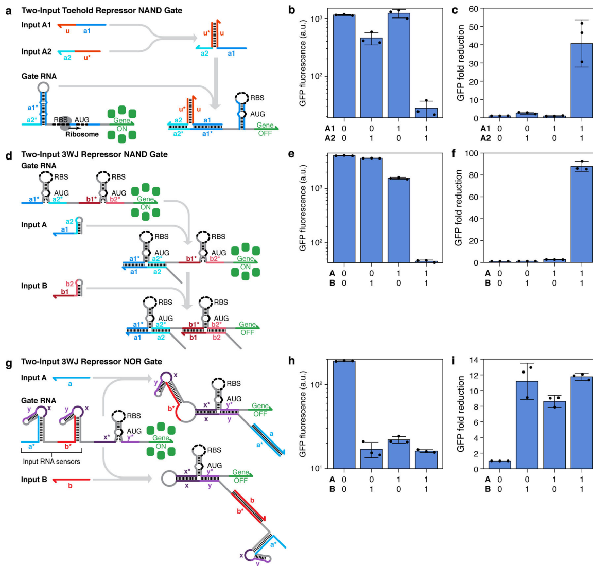
Figure 5 | Two-input logic operations using repressor-based devices.
