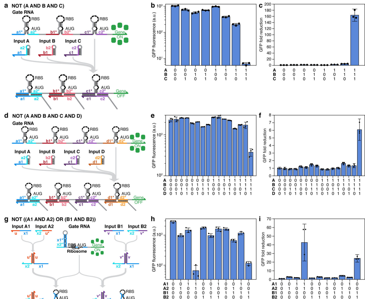
Figure 6 | Multi-input ribocomputing devices employing toehold and 3WJ repressors. a , Design of a three-input 3WJ repressor NAND gate. The gate RNA contains three orthogonal 3WJ repressor hairpins in-frame and upstream of the output gene. b , c , GFP fluorescence ( b ) and fold reduction ( c ) for the three-input 3WJ repressor NAND device. d , Design of a four-input 3WJ repressor NAND gate. The gate RNA contains four orthogonal 3WJ repressor hairpins in-frame and upstream of the output gene. e , f , GFP fluorescence ( e ) and fold reduction ( f ) for the four-input 3WJ repressor NAND device. g , Design of a NOT ((A1 AND A2) OR (B1 AND B2)) logic circuit based on toehold repressors. Independent two-input NAND gate behavior is enabled by two partial-trigger domains x1 and x2 coupled with bridging domains u and u* for inputs A1 and A2 or with orthogonal bridging domains v and v* for inputs B1 and B2. The two partial-triggers present the full-length trigger for the toehold repressor. h , i , GFP fluorescence ( h ) and fold reduction ( i ) for the four-input ribocomputing device based on toehold repressors. Devices were measured 6 hr after induction. GFP fluorescence values and their error bars are the arithmetic mean and SD, respectively, of n=3 biologically independent samples. Fold reductions for each device were calculated by dividing the GFP fluorescence value from the gate RNA obtained for the null input case by the GFP fluorescence value for each input combination. Relative errors for the fold reductions were obtained by adding the relative fluorescence errors in quadrature.
