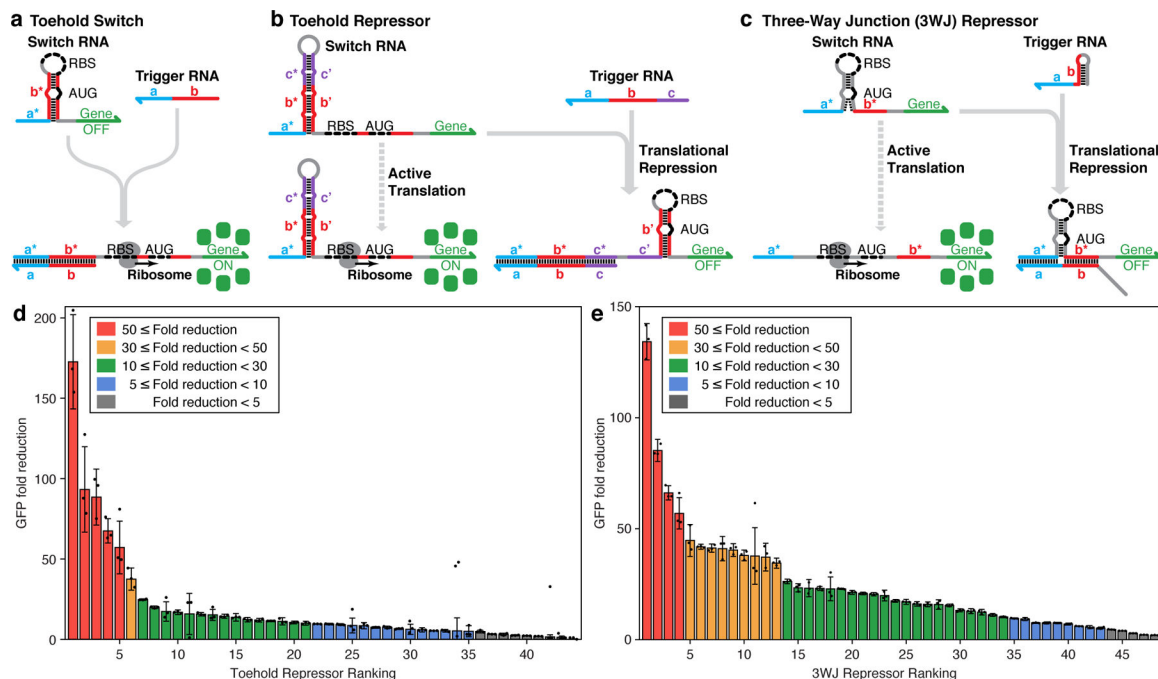
Figure 1 | Operating mechanisms of de-novo -designed repressors and in vivo characterization. a , Toehold switches repress translation through base pairs before and after the start codon (AUG). Interactions are initiated via a single-stranded toehold domain a* in the switch RNA that binds to a complementary a domain on the trigger RNA. A branch migration through domain b frees the ribosomal binding site (RBS) and start codon to allow translation. b , Toehold repressors harbor a strong hairpin structure upstream of an exposed RBS and start codon for translation of a downstream gene. The toehold domain a* of the switch binds to the trigger, initiating a branch migration that opens the strong hairpin stem. Newly freed domains form a hairpin structure that represses translation. c , The switch RNA of a three-way junction (3WJ) repressor contains an unstable hairpin structure that allows ribosomal access to the RBS and start codon and two single-stranded domains a* and b* for trigger binding. The trigger RNA employs a toehold to bind to the switch RNA and establish a three-way junction structure that prevents ribosomal access to the RBS and start codon. d , Fold reduction of GFP fluorescence levels obtained 3 hr after induction for 44 first-generation toehold repressors. e , Fold reduction of GFP fluorescence levels obtained 3 hr after induction for 48 3WJ repressors. Fold reduction is the ratio of the arithmetic mean of the GFP fluorescence level for the ON and OFF translation states. The relative errors for the ON and OFF states are from the SD of n=3 biologically independent samples. Relative errors for GFP fold reduction were obtained by adding the relative errors of the repressor ON- and OFF-state fluorescence measurements in quadrature. Individual points show the fold reduction from n=3 pairs of biologically independent samples.
