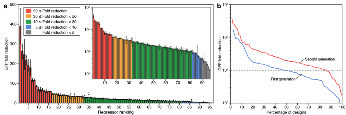
Figure 2 |. Characterization of forward-engineered toehold repressors.
