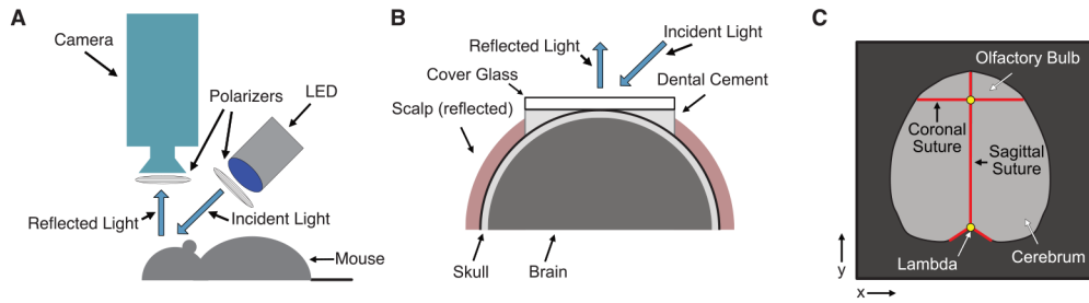
Fig. 1. Schematic of the optical intrinsic signal (OIS) imaging system. (A) Diagram of system components and light path. (B) Cross-section of the mouse head during imaging. (C) Schematic of the field-of-view demonstrating the goal of segmentation. The exposed brain is shown in light gray, with surrounding hair and skin in dark gray. Major suture landmarks are shown in red. Points used for the atlas affine transformation are in yellow.
