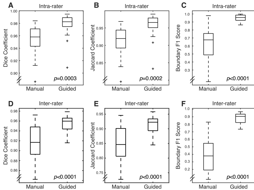
Fig. 7. Box plots for measures of segmentation reliability. For all metrics, guided segmentation decreased variation for both intra- and inter-rater segmentation. (A) Dice coefficient for intra-rater segmentation. (B) Jaccard coefficient for intra-rater segmentation. (C) Boundary F1 score for intra-rater segmentation. (D-F) Same as A-C for inter-rater segmentation.
