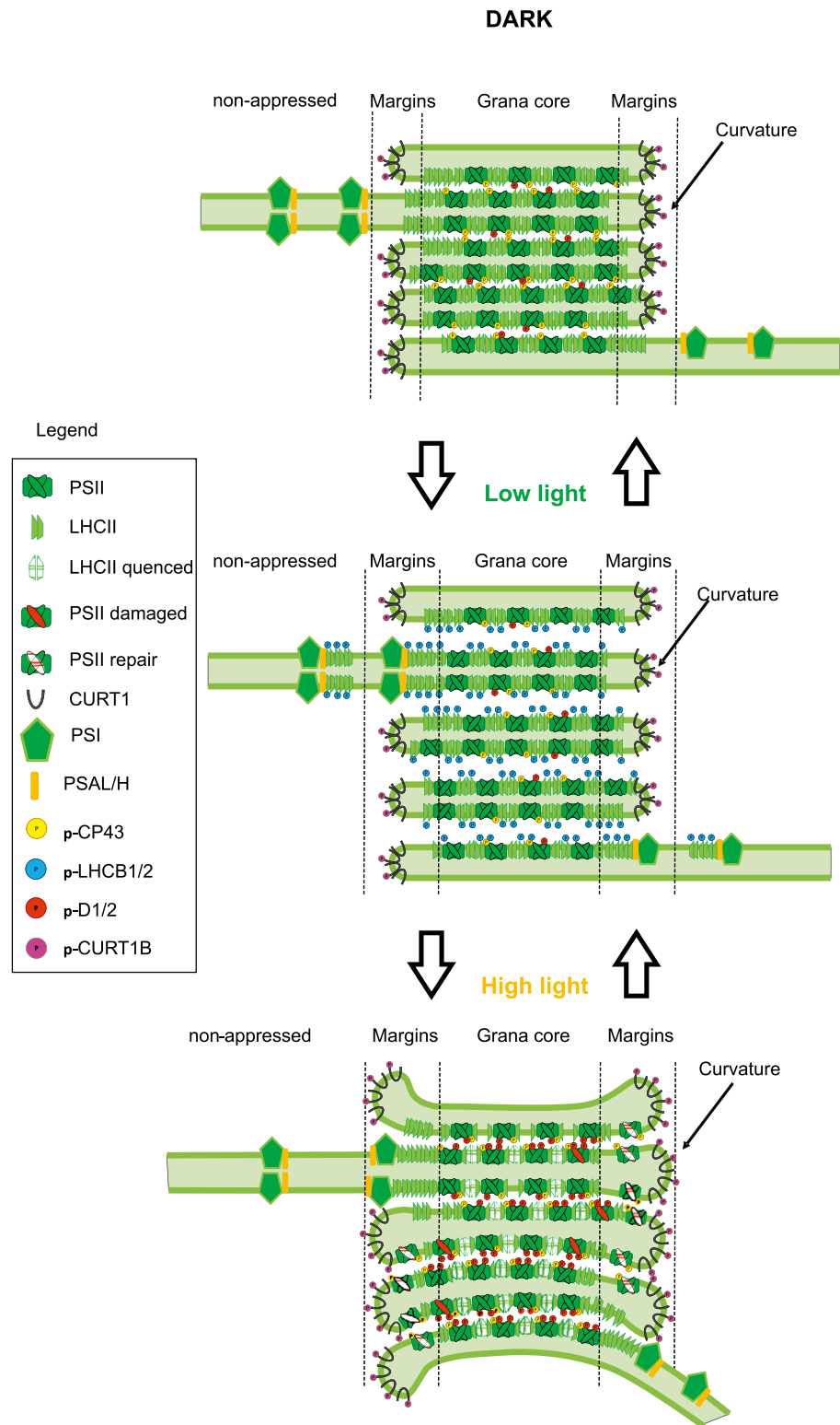
Figure 8. Scheme of the interaction of the phosphorylation of PSII core, LHCII, and CURT1B. The transition from dark to LL leads to an increase in LHCII phosphorylation and a decrease in CP43 phosphorylation. Consequently, loosening of the appressed grana stacks, and thus widening of the size of the partition gaps, occurs. The increased interaction of phosphorylated LHCII with PSI in the loosely appressed membranes results in increased area of the margin domain. The shift from LL to HL results in a decrease of the size of the partition gaps between grana core thylakoid membranes due to both dephosphorylation of LHCII and increased phosphorylation of PSII core proteins. The increased CURT1B phosphorylation, instead, promotes outward bending of the edges of grana margins (curvature domain), which accommodates the PSII repair cycle. The scheme is based on the results presented in this paper and in previous literature (Chow et al., 2005; Tikkanen et al., 2008a, 2008b; Fristed et al., 2010; Dietzel et al., 2011; Anderson et al., 2012; Grieco et al., 2012, 2015; Armbruster et al., 2013; Wientjes et al., 2013; Yamamoto et al., 2013; Tikkanen and Aro, 2014; Yoshioka-Nishimura et al., 2014; Suorsa et al., 2015; Yokono et al., 2015, 2019; Bos et al., 2017; Puthiyaveetil et al., 2017; Schwarz et al., 2018; Johnson and Wientjes, 2019; Wood et al., 2019).
