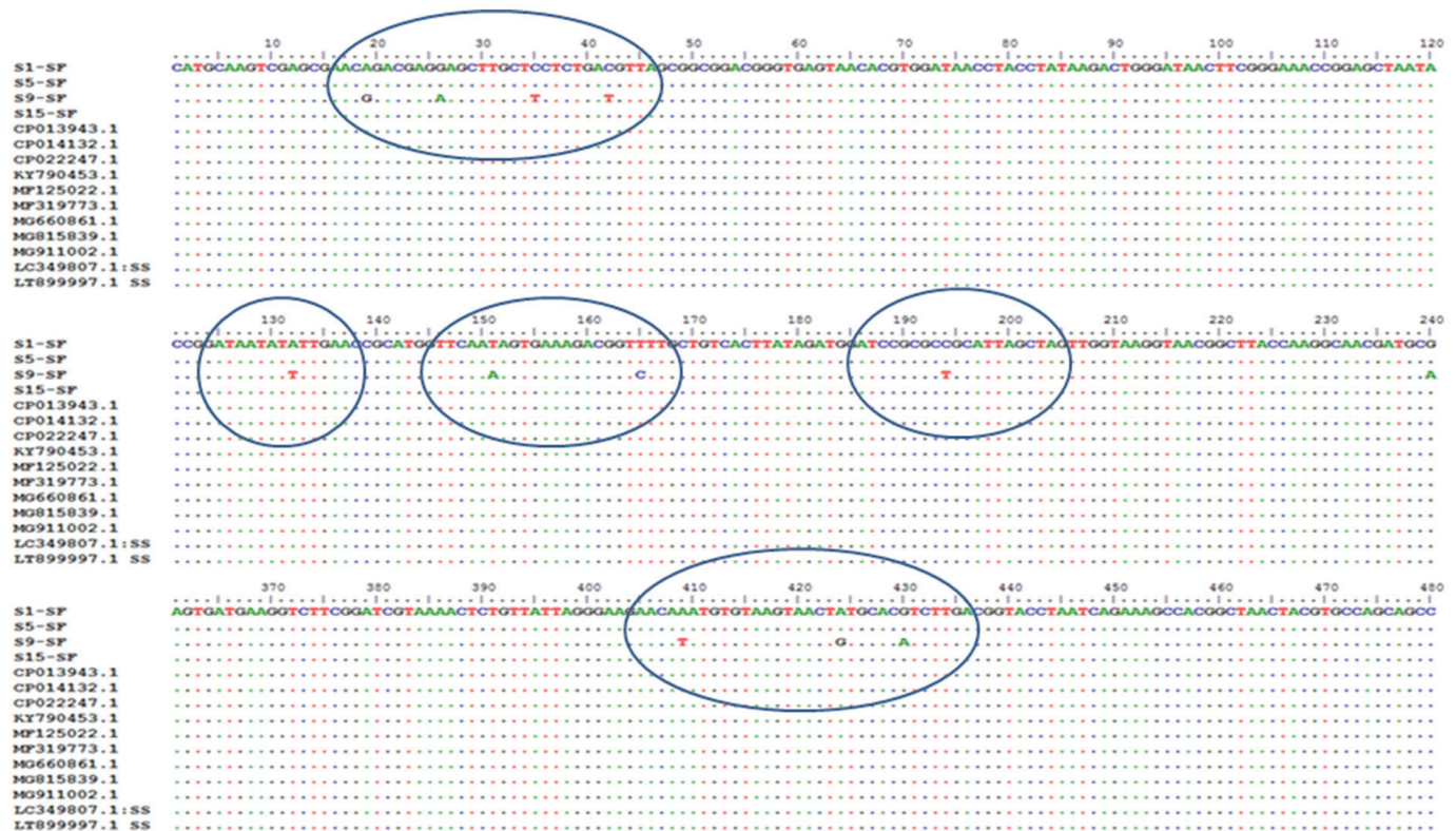
Figure 1. Multiple sequence alignments of 16S rRNA genes. Dots represent residues identical to the nucleotide in the top sequence. S1-SF: S. epidermidis isolated from dairy food; S5-SF: S. epidermidis isolated from hand swabs of food handlers; S15-SF: S. epidermidis isolated diarrheal swabs of patients and S9-SF: S. epidermidis isolated from nasal swabs of patients.
