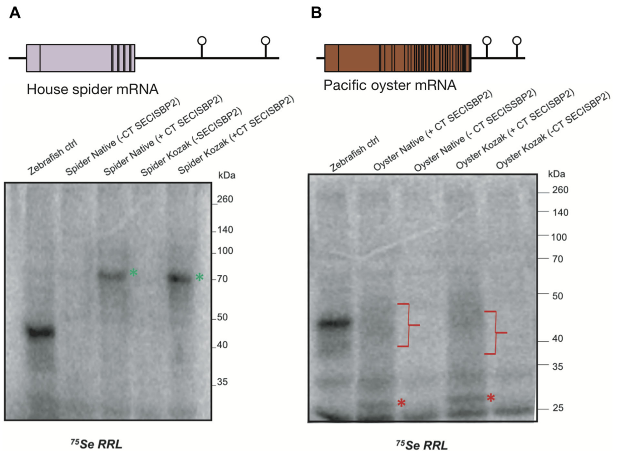
Fig 4. Invertebrate SelenoP mRNA translation in CT-SECISBP2 supplemented RRL.
