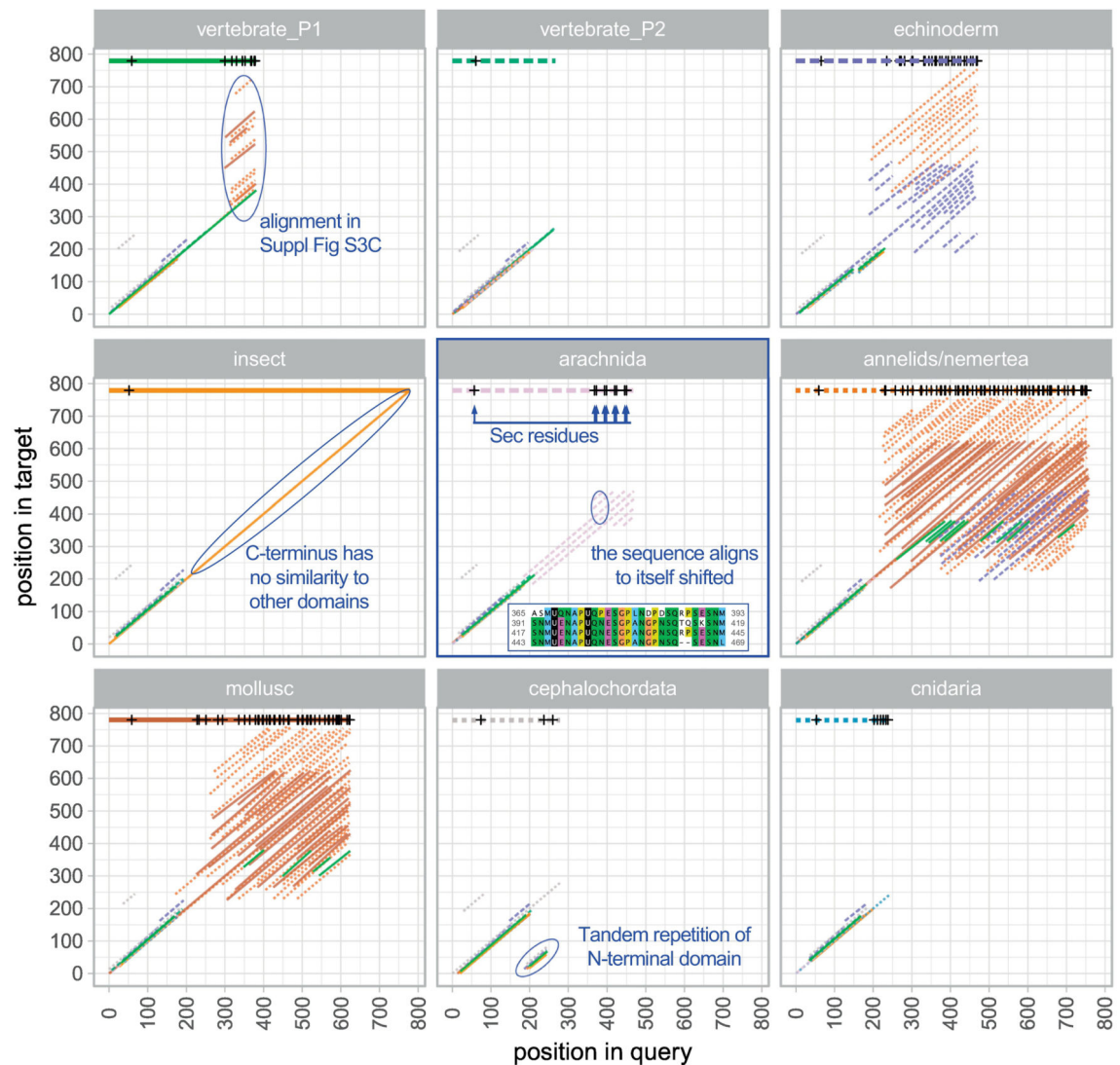
Fig 3. Homology and modularity in SelenoP protein sequences.
