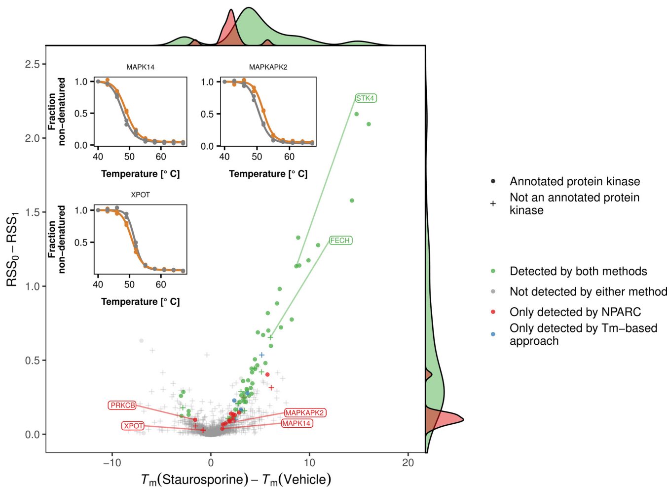
FIG. 4. NPARC is sensitive to small but reproducible T_m -shifts. The plot compares the effect size measure used by NPARC, namely RSS_0 - RSS_1 (y axis), to the T_m -difference (x axis) for those proteins in the staurosporine data set for which T_m estimates could be obtained. Proteins with Benjamini-Hochberg adjusted p values \leq 0.01 are marked in red if they were exclusively found by NPARC, and in green if they were also detected by the T_m -based approach of (6). NPARC detects targets with small T_m -differences if the measurements are reproducible between replicates.
