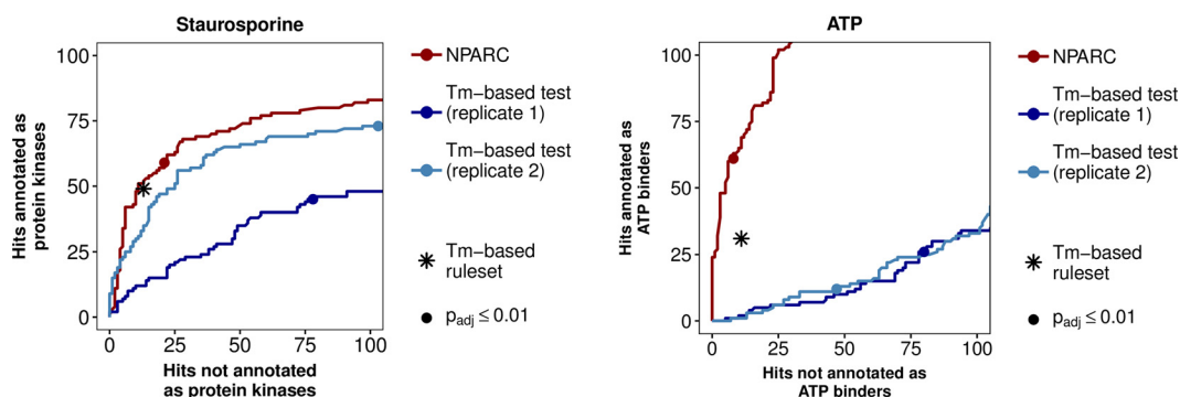
FIG. 5. Sensitivity and specificity. Shown are pseudo-ROC curves, with expected hits (as a proxy for true positives) along the y axis and unexpected hits (as a proxy for false positives) along the x axis. The curves are obtained by varying the p value cutoff of the F -test of NPARC (which is computed across replicates), and of the z -test of the T_m -based approach (6) (which is computed separately for each replicate). The asterisks indicate the result from the decision rules of (6) on the z -test results (Table V). The dots indicate a threshold of 0.01 on the Benjamini-Hochberg adjusted p values from NPARC (derived on both replicates in parallel) and on the Benjamini-Hochberg adjusted p values from the T_m -based approach (computed individually for each replicate). NPARC is modestly better than the T_m -based approach on the staurosporine data (A), and substantially better on the ATP data (B). The proteins found by NPARC at Benjamini-Hochberg adjusted p value \leq 0.01 are also shown in supplemental Figs. S6 and S7.
