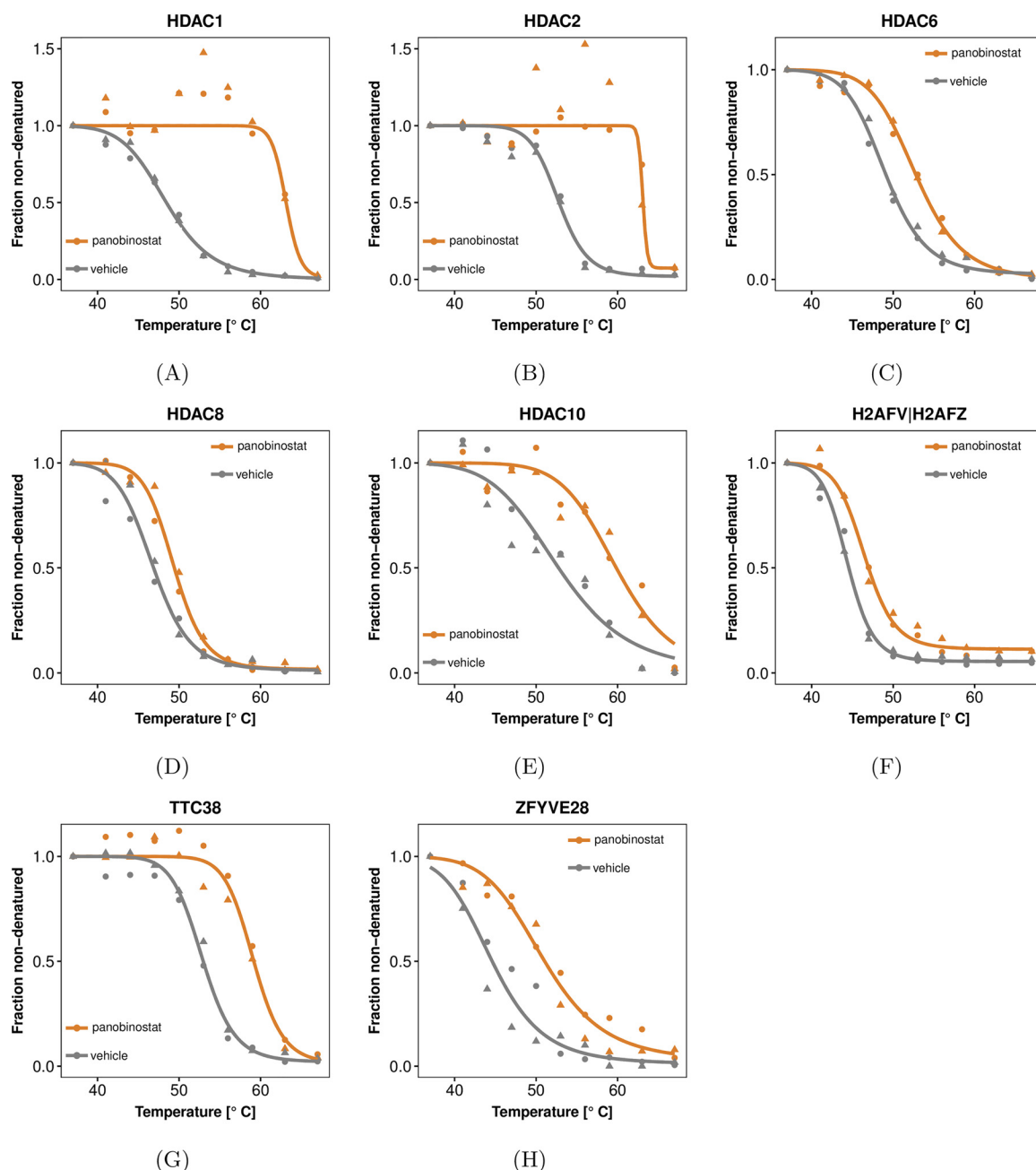
FIG. 3. Direct and indirect targets of the HDAC inhibitor panobinostat detected by NPARC (FDR \leq 0.01 according to the method of Benjamini and Hochberg (26)). A–E, Data and curve fits for five HDACs that show significant shifts in their thermostability. HDAC1 and HDAC2 are not detected by the T_m -based approach of (6), because the higher variance between the replicates of the panobinostat-treated condition leads to them being eliminated by the filter heuristics of that method (Table III). In contrast, NPARC naturally takes the variance into account in the computation of the F -statistic and does not require such filtering steps. F–H, Data and curve fits for known non-HDAC targets.
