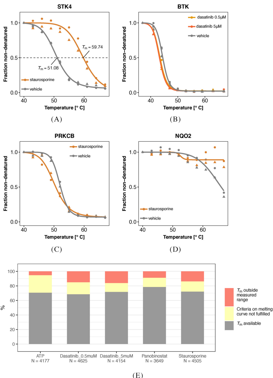
FIG. 1. TPP data analysis challenges. A–D, Examples for protein melting curves with and without drug (see color keys). In each case, ten temperatures were assayed, and two experimental replicates were made per condition, indicated by circle and triangle symbols. Fits of the sigmoid model (Eq. (3)) to both replicates jointly are shown by smooth lines. A, For serine/threonine protein kinase 4 (STK4), the binding of staurosporine is reflected by a marked shift between the curves. The fitted values for the melting points ( T_m ) are shown. B, For Bruton’s tyrosine kinase (BTK), there is a small but reproducible shift between the curves. C, Protein kinase C beta (PRKCB) is destabilized by staurosporine; the effect occurs mainly at lower temperatures. D, NAD(P)H quinone dehydrogenase 2 (NQO2) is strongly stabilized by staurosporine. Although in each case, the effects of drug binding are clearly reproducible between replicates, the T_m -based approach of (6) only detects (A) and misses (B–D). In the case of (B) and (C), the fitted T_m are too similar, so that the statistical test does not assess the difference as significant. In the case of (D), no reasonable estimate for T_m in the staurosporine treated condition can be obtained, as it would lie outside the measured temperature range, and the protein is discarded from the analysis. In contrast, NPARC, the method proposed in this article, detects all four cases. E, The fraction of proteins in each of the data sets of Table I that is missed by the T_m -based approach because of failure to estimate T_m or to meet the goodness-of-fit criterion (Table III).
