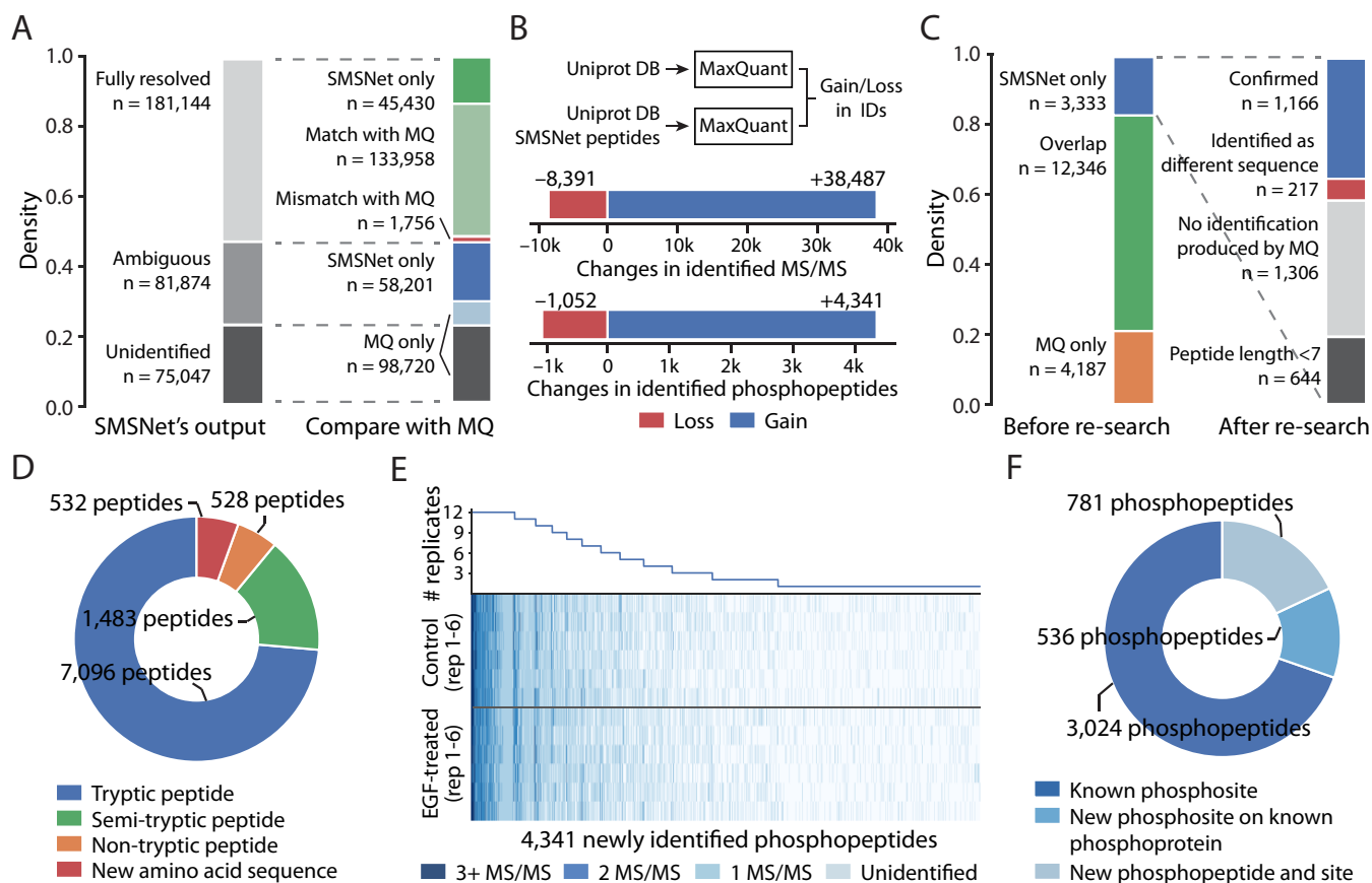
FIG. 5. SMSNet improves the coverage of human phosphoproteome. A , Stacked bar plots showing the numbers of MS/MS spectra identified by SMSNet and the overlaps between SMSNet and prior study (18). B , The gains and losses in number of identified MS/MS spectra and phosphopeptides after adding SMSNet's identifications to the human proteome database and re-analyzing with MaxQuant (see Experimental Procedures). C , Stacked bar plots showing the numbers of phosphopeptides identified by MaxQuant and SMSNet and the numbers of new phosphopeptides that could be confirmed by re-analyzing SMSNet's identifications with MaxQuant. Peptides shorter than 7 amino acids were not considered during the search. "No identification produced by MQ" indicates that none of the MS/MS spectra of a phosphopeptide were identified as peptides by MaxQuant. "Identified as different sequence" indicates that none of the MS/MS spectra of a phosphopeptide were confirmed by MaxQuant as the same identification produced by SMSNet and at least one MS/MS spectrum was identified as a different peptide. D , Pie chart showing the composition of all newly identified peptides gained by adding SMSNet's identifications to MaxQuant's search. This includes phosphopeptide and non-phosphopeptide identifications from all MS/MS spectra that were not previously identified by prior study. It should be noted that because MaxQuant searches were performed with full-tryptic enzyme specificity, all identifications of semi-tryptic peptides, non-tryptic peptides, and peptides with new amino acid sequences were possible because of sequences supplied by SMSNet. E , Heatmap and line plot showing the reproducibility of 4,341 newly identified phosphopeptides after re-analysis using MaxQuant across 6 control and 6 epidermal growth factor (EGF)-treated replicates. Each row in the heatmap corresponds to one mass spectrometry experiment. F , Pie chart showing the overlap between newly identified phosphopeptides and known phosphoproteins and phosphosites in the PhosphoSitePlus database. An identified phosphopeptide was counted as "Known phosphosites" only if all identified phosphorylation sites on that peptide are reported in the database. Identified phosphopeptides that contain unreported phosphosites were grouped based on whether they could be mapped to known phosphoproteins in the database.
