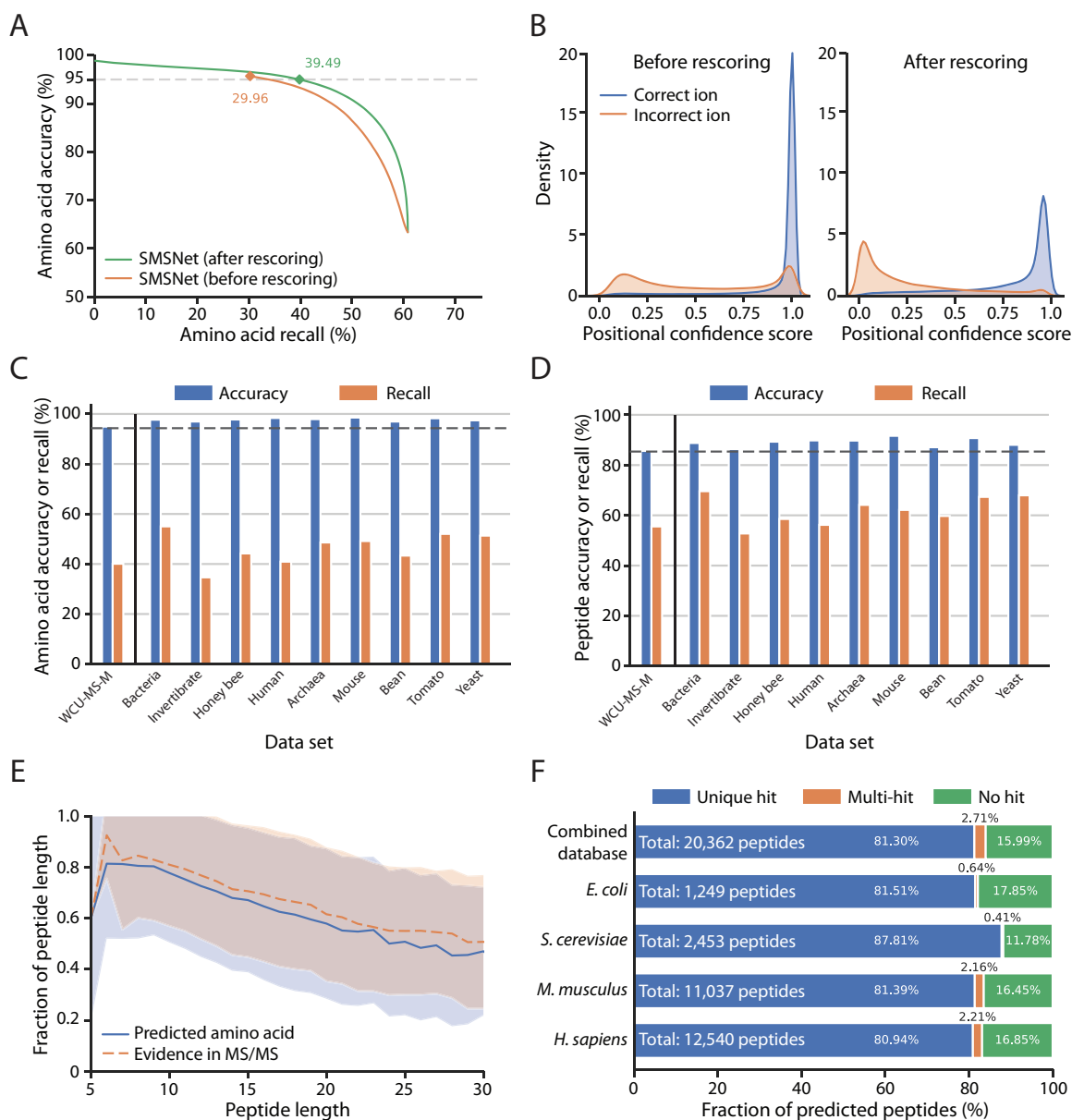
FIG. 3. The Sequence-Mask-Search framework significantly improves de novo peptide sequencing accuracy. The WCU-MS-M dataset was used to train and evaluate the performance of SMSNet here. A , Amino acid-level performances for SMSNet before and after the positional confidence score adjustment step. The corresponding recalls at 5% amino acid false discovery rate are indicated. B , Histograms showing the distributions of positional confidence scores produced by SMSNet before and after score adjustment. C , Bar plots showing amino acid-level accuracies and recalls of SMSNet on a test set derived from WCU-MS-M and on MS/MS spectra of nine species that comprise the dataset curated by DeepNovo's authors. The threshold on positional confidence score was selected so that 5% amino acid false discovery rate was achieved on the WCU-MS-M test set (the leftmost bars). Dashed line indicates the expected 95% accuracy based on the applied score threshold. D , Similar bar plots showing the results at peptide-level. Dashed line indicates the expected accuracy level based on the applied score threshold. E , Line plots comparing the fraction of identified amino acid positions that pass the same score threshold used in C–D in peptides of various lengths (blue line) to the fraction of amino acid positions that can be definitely determined based on observed ions in the MS/MS spectra (orange dashed line). Shaded area indicates the \pm 1 standard deviation range. F , Stacked bar plots showing the fraction of identified peptides that could be matched to various protein sequence databases. Amino acid sequence database for each species was downloaded from UniProt (see Experimental Procedures). Combined database integrates amino acid sequences from all four species considered. In each bar, only identifications whose ground truths exist within the corresponding database were counted. "Unique hit" means that the identified sequence matches to exactly one possibility in the database. "Multi-hit" means that the identified sequence matches to multiple possibilities. "No hit" means the identified sequence does not match to anything in the database.
