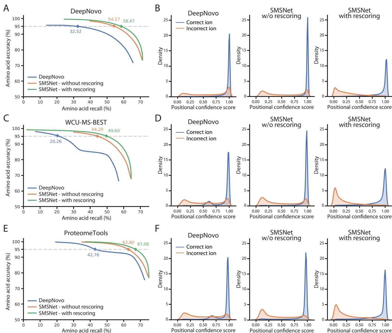
FIG. 2. SMSNet outperforms state-of-the-art de novo peptide sequencing tool. To provide fair comparisons, SMSNet and DeepNovo were retrained using the same high-resolution MS/MS spectra from the indicated datasets. Furthermore, as DeepNovo does not include post-processing, the performance of SMSNet with and without re-scoring are shown together here. A , Amino acid-level performances for SMSNet and DeepNovo when evaluated on the dataset curated by DeepNovo's authors. The corresponding recalls at 5% amino acid false discovery rate are indicated. B , Histograms showing the distributions of positional confidence scores produced by SMSNet and DeepNovo when evaluated on the dataset curated by DeepNovo's authors. C–D , Similar plots showing performances of SMSNet and DeepNovo when evaluated on our WCU-MS-BEST dataset. E–F , Similar plots showing performances of SMSNet and DeepNovo when evaluated on high-quality MS/MS spectra of synthetic peptides acquired from ProteomeTools database.
