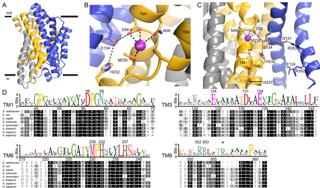
Figure 6. A network of highly conserved charged and protonatable residues adjoins the metal-binding site. (A) Crystal structure of DraNrap in an outward-open conformation bound to Mn^{2+} (magenta sphere; PDB accession no. 6BU5; Bozzi et al., 2019). TMs 1, 5, 6, and 10 are gold; TMs 2, 7, and 11 are gray; and TMs 3, 4, 8, and 9 are blue. (B) D56, N59, M230, and the A53 carbonyl coordinate Mn^{2+} in the outward-open state, along with two waters (not depicted). (C) View from the plane of the membrane of a network consisting of E134, H232, D131, R353, R352, and E124 that extends \sim 20 Å from D56 to the cytosol. TMs 8 and 4–5, in front of TMs 3 and 9, respectively, were removed for clarity. (D) Sequence logos from an alignment of 6,878 Nrap sequences. All 10 mutated residues (numbers above) are highly conserved. Canonical helix-breaking motifs at the metal-binding site are DPGN in TM1 and MPH in TM6. TM6's H237 is a glycine in many fungal homologues. The second TM9 arginine (R353) varies in location (*) due to an extra helical turn in many homologues; this insertion contains a third arginine in some homologues. See also Fig. S4.
