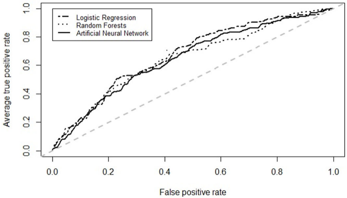
Figure 2. Average receiver operating characteristic curves for machine learning models predicting need for glaucoma surgery within 6 months among patients with primary open-angle glaucoma using systemic data in the electronic health record.
