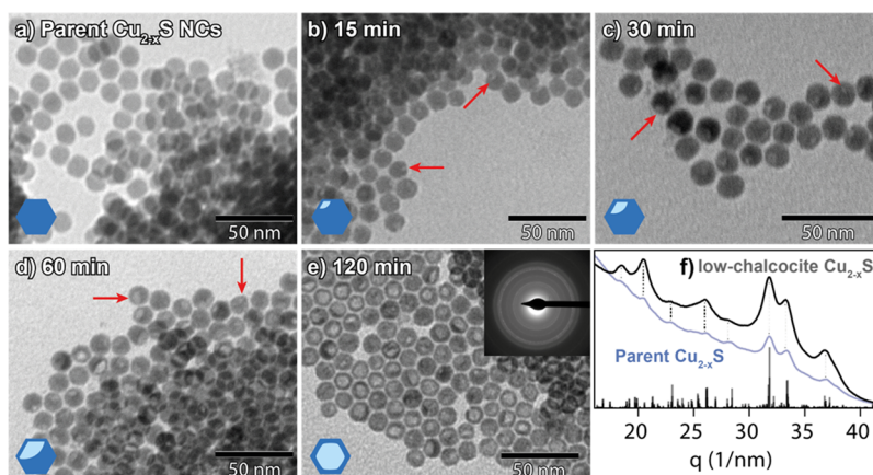
Figure 2. TEM images of (a) parent \text{Cu}_{2-x}\text{S} NCs and (b–e) product NCs obtained after reacting the NCs shown in (a) with \text{GaCl}_3 at 30\text{ }^\circ\text{C} for (b) 15 min, (c) 30 min, (d) 60 min, and (e) 120 min. Red arrows indicate regions of low contrast within the nanocrystals (cartoons in the lower-left corner give an impression of the observed contrast in the NCs). Top-right inset in (e) depicts an electron diffraction pattern of the corresponding sample. Panel (f) is the azimuthally integrated ED pattern depicted in (e). Reference bars in (f) are calculated patterns based on the low-chalcocite \text{Cu}_{2-x}\text{S} crystal structure described in ref 34. The blue curve in (f) corresponds to the PED pattern of the parent \text{Cu}_{2-x}\text{S} nanocrystals. Dotted lines serve as guides for the eye.
