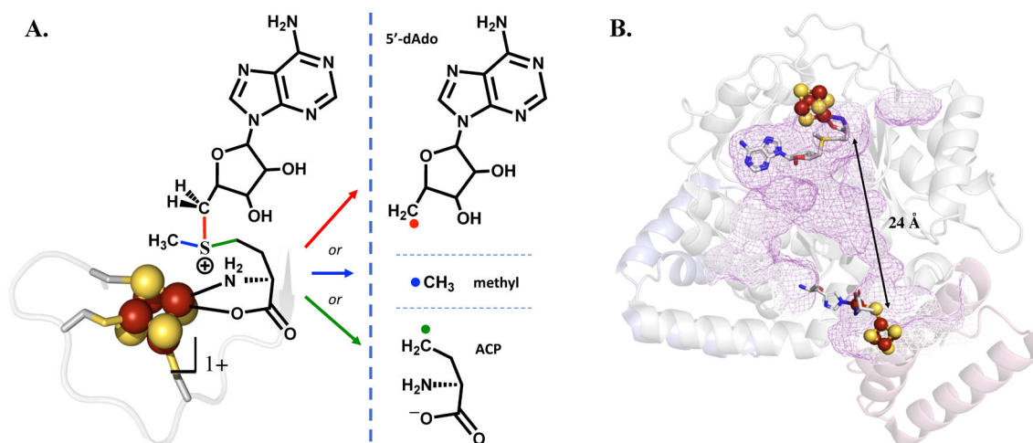
Figure 1. Reductive cleavage of SAM and the structure of HydG. (A) The SAM-cluster interaction in RS enzymes (left), and the three different radical products that can result from reductive S–C bond cleavage in SAM (right). Canonical RS enzymes cleave the S–C5' bond (red) to generate the 5'-dAdo• radical intermediate, while the noncanonical RS enzyme Dph2 cleaves the S–C( \gamma ) bond (green) to yield an ACP radical fragment that adds to substrate. (B) Overview of the structure of HydG (PDB 4WCX), with the radical SAM cluster (top) and the auxiliary cluster (bottom) connected by a long active site tunnel (purple mesh).
