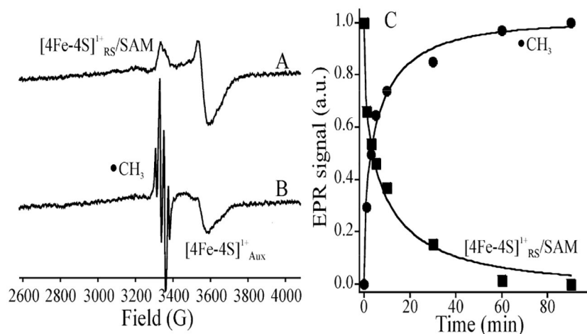
Figure 2. X-band EPR spectra of (A) [4\text{Fe-4S}]^+ + \text{SAM} HydG complex before and (B) after photolysis at 12 K with 450 nm LED for 1 h. (C) Time course for decay of [4\text{Fe-4S}]^+ + \text{SAM} (■) upon photolysis monitored at 3640 G, and increase of \bullet\text{CH}_3 (●) monitored at 3306 G. The photo reaction appears to be complete at ~90 m, as the EPR spectrum does not change upon further photolysis. The two progress curves are then normalized and fit to stretched-exponential decay, I = \exp(-[t/\tau]^n) , and rise, I = 1 - \exp(-[t/\tau]^n) , functions with the same parameters, \tau = 7 \pm 1 min and n = 0.52 \pm 0.02 . In (B), the unchanged signal from [4\text{Fe-4S}]_{\text{AUX}}[(\text{Cys})\text{Fe}] cluster and that from \bullet\text{CH}_3 are both identified. EPR conditions: microwave frequency, 9.38 GHz; modulation 10 G; T = 12 K.
