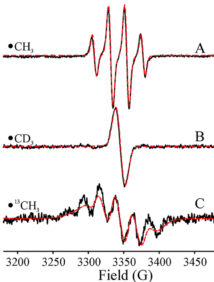
Figure 3. EPR spectra (black) and simulations (red). (A) Spectrum of rapidly tumbling \bullet\text{CH}_3 generated with natural abundance SAM, obtained by subtraction of the properly scaled signal from the persistent signal (see text). (B) \bullet\text{CD}_3 generated with methyl- d_3 -SAM. (C) \bullet^{13}\text{CH}_3 generated with ^{13}\text{C} -methyl-SAM. Conditions: T = 40 K, modulation amplitude, 5 G; see Figure 4 for spectra with lower modulation. EasySpin simulation parameters: function, chili ; \mathbf{g} = [2.0015, 2.0015, 2.0055, ] , ( g_{\text{iso}} = 2.003 ). For spectra (A) and (C), A(^1\text{H}_{a,b,c}) = -[86, 44, 62] MHz ( a_{\text{iso}}(^1\text{H}_{a,b,c}) = -63.3 MHz), (\alpha, \beta, \gamma) = (120, 0, 0) for 1Ha, (\alpha, \beta, \gamma) = (-120, 0, 0) for 1Hb, (\alpha, \beta, \gamma) = (0, 0, 0) for 1Hc; for spectrum (C), A(^{13}\text{C}) = [-10, -10, 260] MHz. \tau_{\text{C}} = 3.2 ns; uniform Gaussian line widths 21 MHz.
