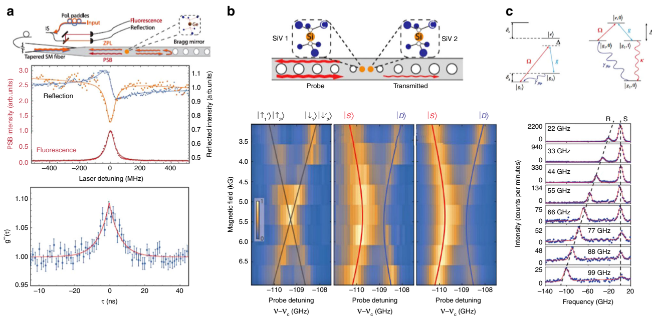
Fig. 4 Quantum optics with group IV colour centres. a Homodyne interferometry with a single GeV centre (top panel). Interference between GeV resonance fluorescence and near-resonant excitation laser light reflected in the fibre by the Bragg mirror. Varying their relative amplitude and phase, by modifying the polarization of the input laser, results in the change in line shape of the output light (mid panel), corresponding to destructive interference (orange) to dispersive (blue). The Hanbury Brown-Twiss interferometry measurement (bottom panel) shows g^2(0) > 1 due to interference between the excitation laser and the resonant fluorescence from the single GeV centre. It highlights the quantum nonlinear character of the coupled GeV-waveguide system (reprinted with permission from ref. 103 . Copyright 2017 by the American Physical Society). b Coherent coupling between two SiV - centres in a photonic crystal cavity. The characteristic avoided crossing (mid panel) indicates a coupling greater than the optical linewidth (from ref. 85 . Reprinted with permission from AAAS). c Widely tuneable Raman emission from a SiV - centre coupled to a photonic crystal cavity (reprinted with permission from ref. 104 . Copyright 2018 by the American Physical Society).
