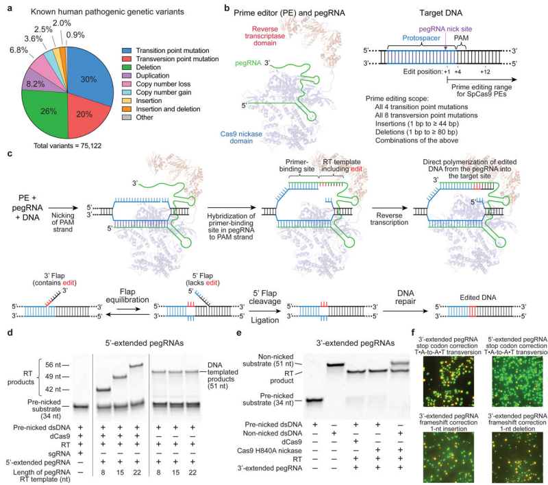
Figure 1. Overview of prime editing and feasibility studies in vitro and in yeast cells. (a) The 75,122 known pathogenic human genetic variants in ClinVar (accessed July, 2019), classified by type. (b) A prime editing complex consists of a prime editor (PE) protein containing an RNA-guided DNA-nicking domain, such as Cas9 nickase, fused to a reverse transcriptase domain and complexed with a prime editing guide RNA (pegRNA). The PE:pegRNA complex enables a variety of precise DNA edits at a wide range of positions. (c) The PE:pegRNA complex binds the target DNA and nicks the PAM-containing strand. The resulting 3' end hybridizes to the primer-binding site, then primes reverse transcription of new DNA containing the desired edit using the RT template of the pegRNA. Equilibration between the edited 3' flap and the unedited 5' flap, cellular 5' flap cleavage and ligation, and DNA repair results in stably edited DNA. (d) In vitro primer extension assays with 5'-extended pegRNAs, pre-nicked dsDNA substrates containing 5'-Cy5 labeled PAM strands, dCas9, and a commercial M-MLV RT variant (RT, Superscript III). dCas9 was complexed with pegRNAs, then added to DNA substrates along with the indicated components. After 1 hour, reactions were analyzed by denaturing PAGE, visualizing Cy5 fluorescence. (e) Primer extension assays performed as in (d) using 3'-extended pegRNAs pre-complexed with dCas9 or Cas9 H840A nickase, and pre-nicked or non-nicked dsDNA substrates. (f) Yeast colonies transformed with GFP–mCherry fusion reporter plasmids edited in vitro with pegRNAs, Cas9 nickase, and RT. Plasmids containing nonsense or frameshift mutations between GFP and mCherry were edited with pegRNAs that restore mCherry translation via transversion, 1-bp insertion, or 1-bp deletion. GFP and mCherry double-positive cells (yellow) reflect successful editing. Images in (d-f) are representative of n=2 independent replicates. For gel source data, see Supplementary Figure 1.
