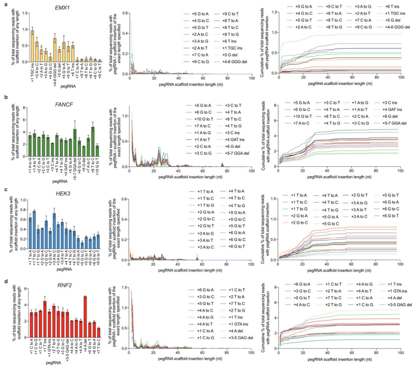
Extended Data Figure 7. Incorporation of pegRNA scaffold sequence into target loci. HTS data were analyzed for pegRNA scaffold sequence insertion as described in Supplementary Note 4. (a) Analysis for the EMX1 locus. Shown is the % of total sequencing reads containing one or more pegRNA scaffold sequence nucleotides within an insertion adjacent to the RT template (left); the percentage of total sequencing reads containing a pegRNA scaffold sequence insertion of the specified length (middle); and the cumulative total percentage of pegRNA insertion up to and including the length specified on the X axis. (b) As in (a) for FANCF . (c) As in (a) for HEK3 . (d) As in (a) for RNF2 . Values and error bars reflect mean±s.d. of n=3 independent biological replicates.
