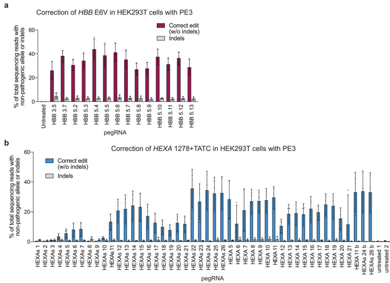
Extended Data Figure 9. PE3-mediated HBB E6V correction and HEXA 1278+TATC correction by various pegRNAs. (a) Screen of 14 pegRNAs for correction of the HBB E6V allele in HEK293T cells with PE3. All pegRNAs evaluated convert the HBB E6V allele back to wild-type HBB without the introduction of any silent PAM mutation. (b) Screen of 41 pegRNAs for correction of the HEXA 1278+TATC allele in HEK293T cells with pE3 or PE3b. Those pegRNAs labeled HEXAs correct the pathogenic allele by a shifted 4-bp deletion that disrupts the PAM and leaves a silent mutation. Those pegRNAs labeled HEXA correct the pathogenic allele back to wild-type. Entries ending in “b” use an edit-specific nicking sgRNA in combination with the pegRNA (the PE3b system). Values and error bars reflect mean \pm s.d. of n=3 independent biological replicates.
