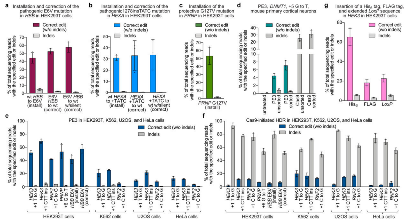
Figure 5. Prime editing of pathogenic mutations, prime editing in primary mouse cortical neurons, and comparison of prime editing and HDR in four human cell lines. (a) Installation (via T•A-to-A•T transversion) and correction (via A•T-to-T•A transversion) of the pathogenic E6V mutation in HBB in HEK293T cells. Correction either to wild-type HBB , or to HBB containing a PAM-disrupting silent mutation, is shown. (b) Installation (via 4-bp insertion) and correction (via 4-bp deletion) of the pathogenic HEXA 1278+TATC allele in HEK293T cells. Correction either to wild-type HEXA , or to HEXA containing a PAM-disrupting silent mutation, is shown. (c) Installation of the protective G127V variant in PRNP in HEK293T cells via G•C-to-T•A transversion. (d) Installation of a G•C-to-T•A transversion in DNMT1 of mouse primary cortical neurons using a split-intein PE3 lentivirus system (see Methods). Sorted values reflect editing or indels from GFP-positive nuclei, while unsorted values are from all nuclei. (e) PE3 editing and indels or (f) Cas9-initiated HDR editing and indels at endogenous genomic loci in HEK293T, K562, U2OS, and HeLa cells. (g) Targeted insertion of a His 6 tag (18 bp), FLAG epitope tag (24 bp), or extended LoxP site (44 bp) in HEK293T cells by PE3. Editing efficiencies reflect sequencing reads that contain the intended edit and do not contain indels among all treated cells, with no sorting, except where specified in (e). Values and error bars reflect mean±s.d. of n=3 independent biological replicates.
