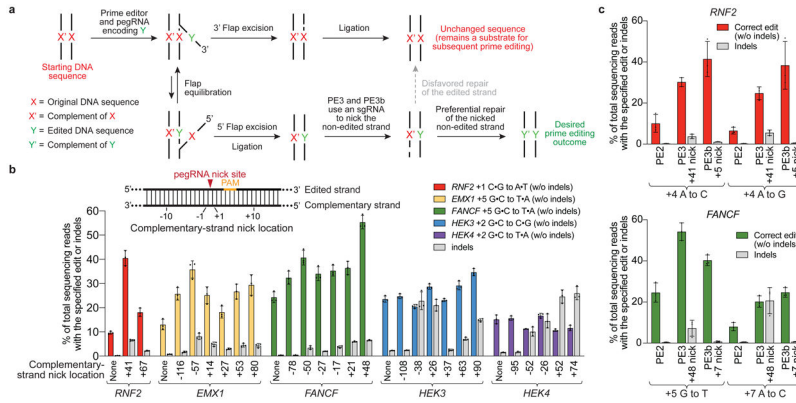
Figure 3. PE3 and PE3b systems nick the non-edited strand to increase prime editing efficiency.
